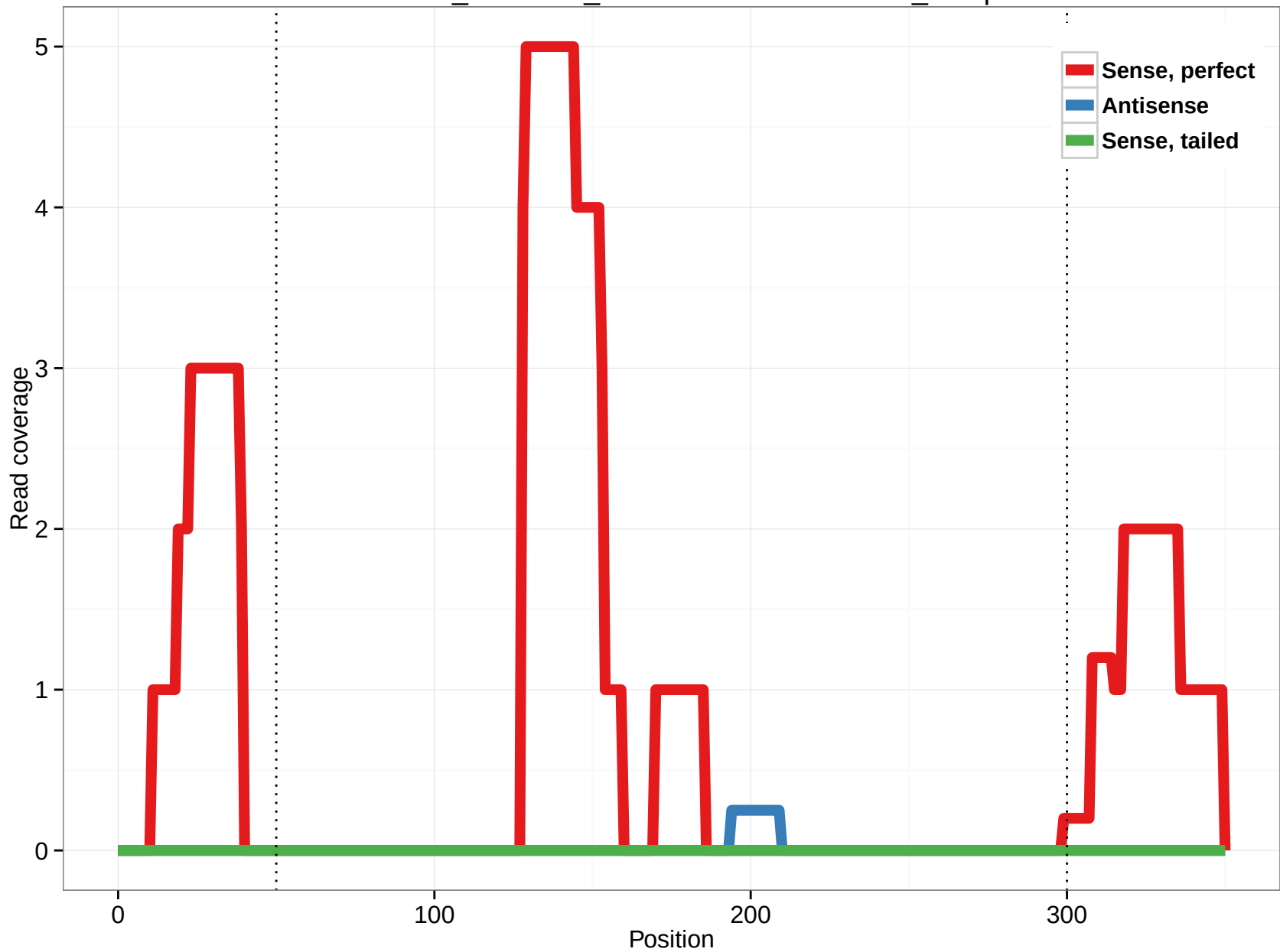
ornAna1_ensGene_ENSOANT00000008159_15.5p
