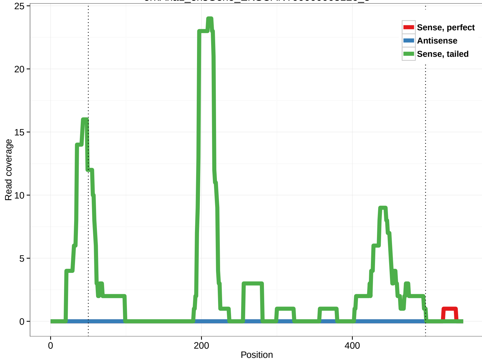
ornAna1_ensGene_ENSOANT00000008126_8
