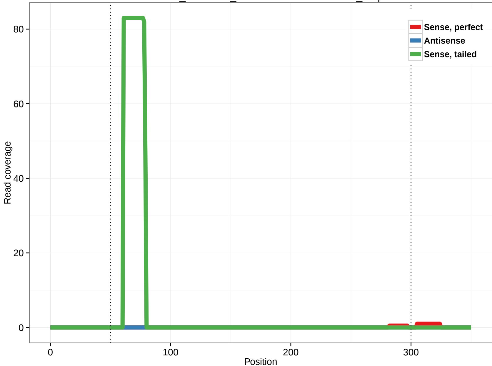
ornAna1_ensGene_ENSOANT00000008099_4.3p
