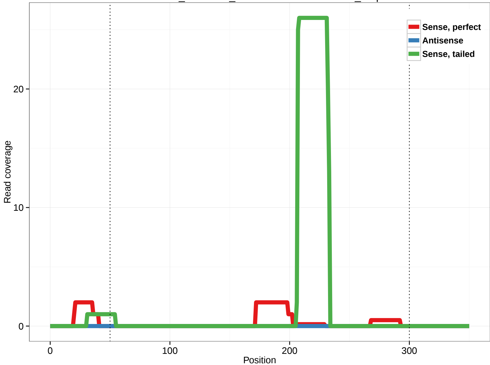
ornAna1_ensGene_ENSOANT00000008063_9.5p
