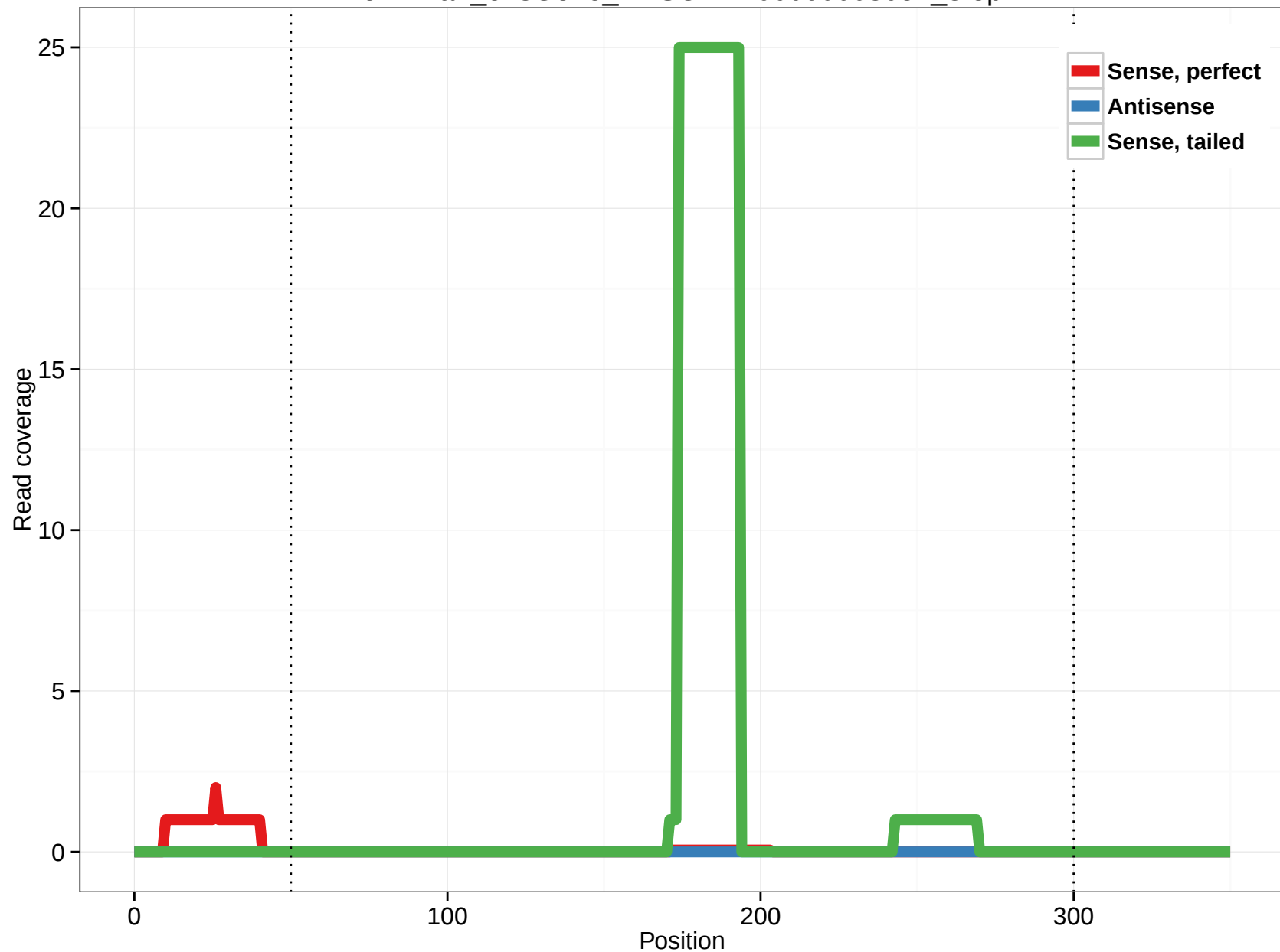
ornAna1_ensGene_ENSOANT00000008057_3.5p
