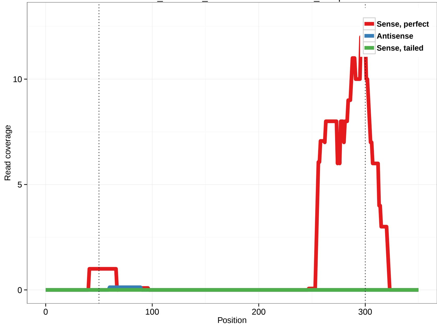
ornAna1_ensGene_ENSOANT00000008012_10.5p
