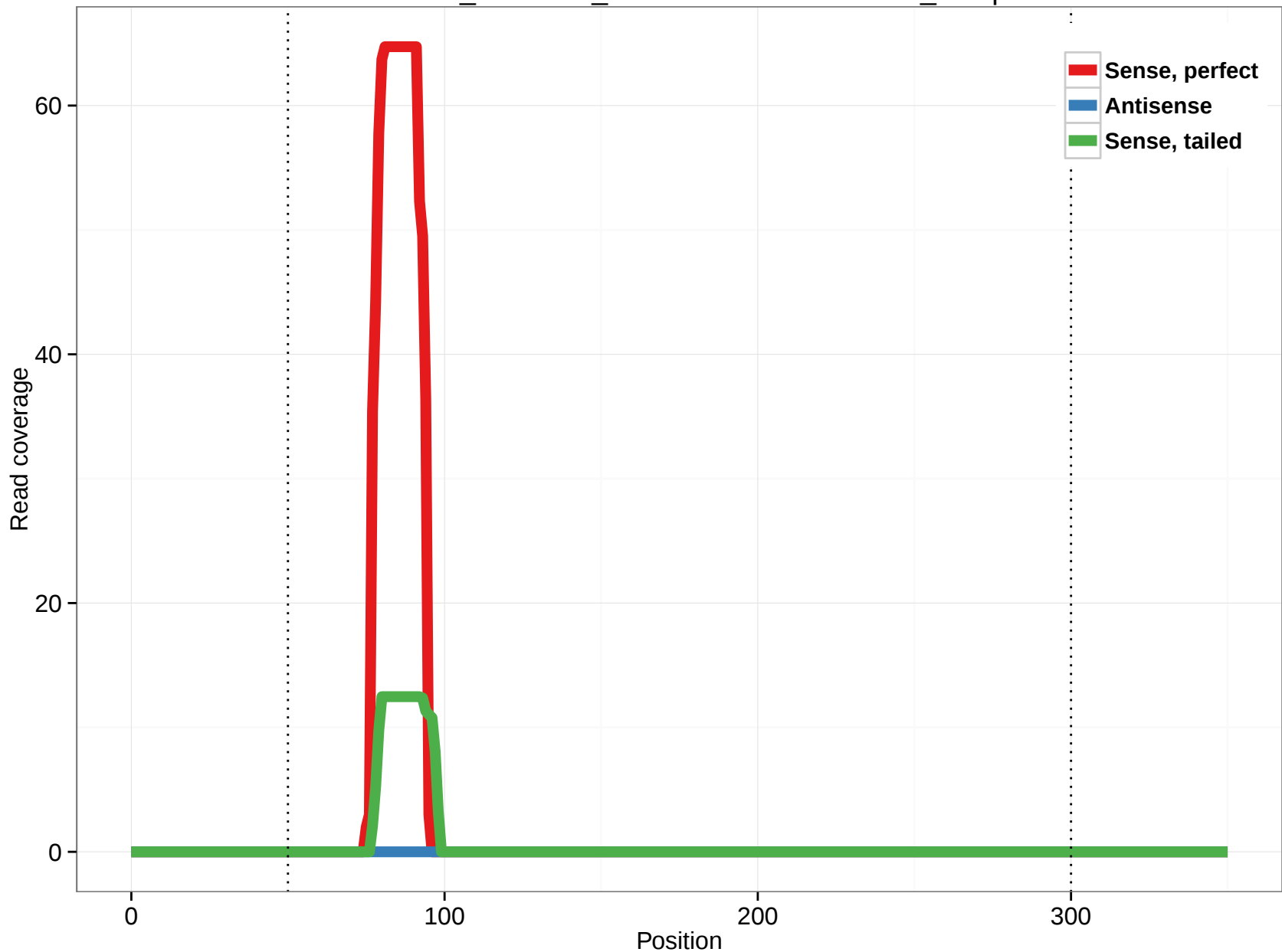
ornAna1_ensGene_ENSOANT00000008011_22.3p
