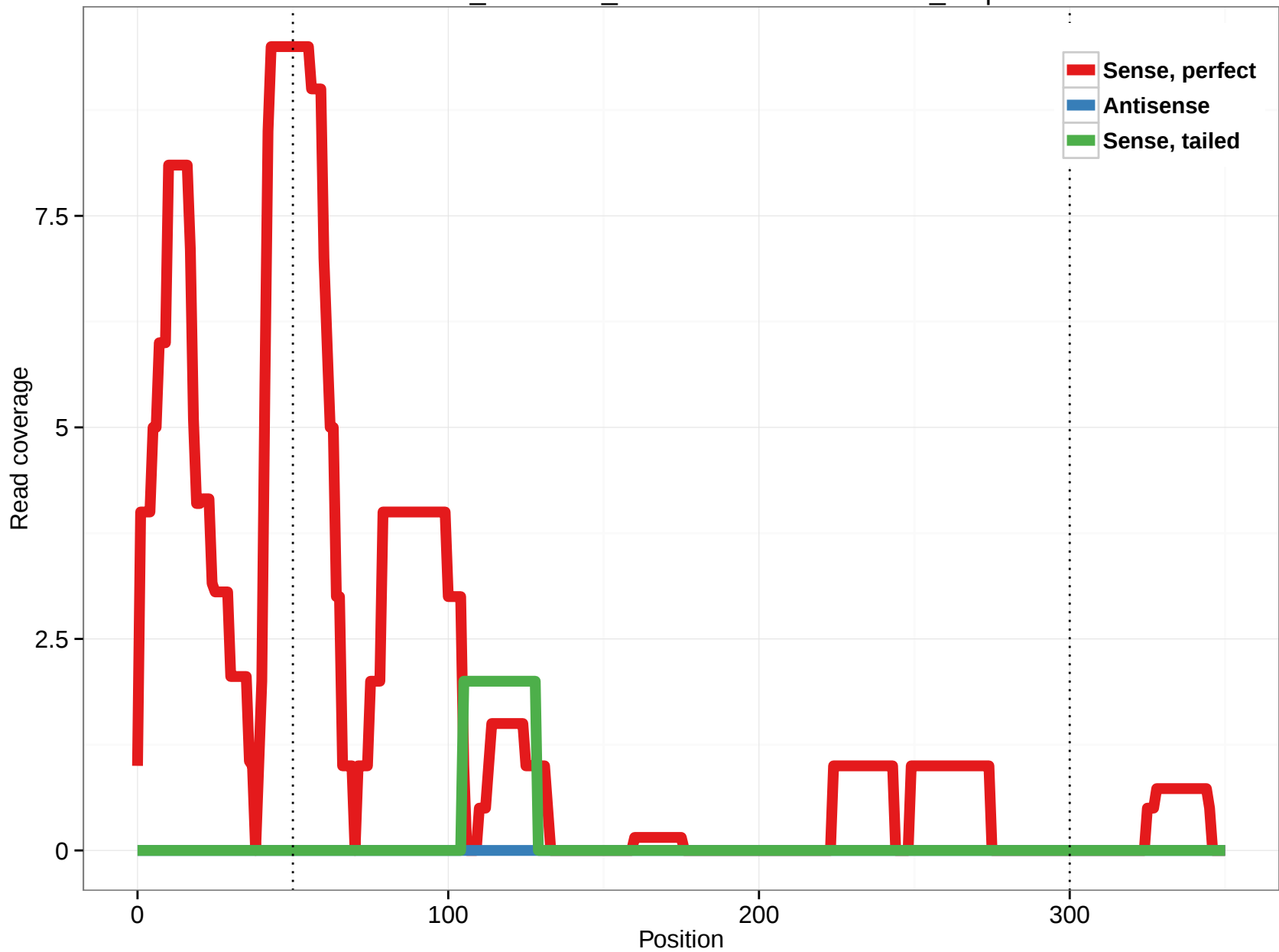
ornAna1_ensGene_ENSOANT00000007983_8.5p
