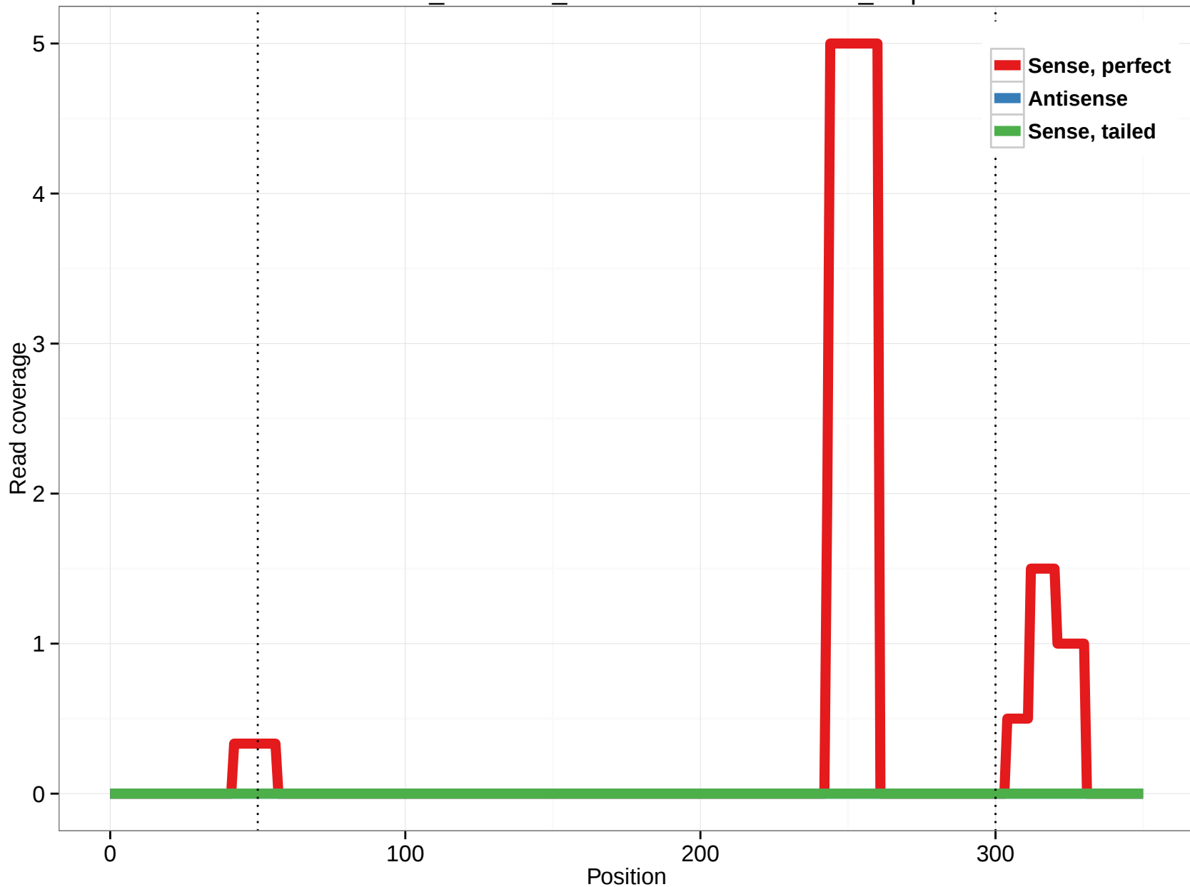
ornAna1_ensGene_ENSOANT00000007982_4.3p
