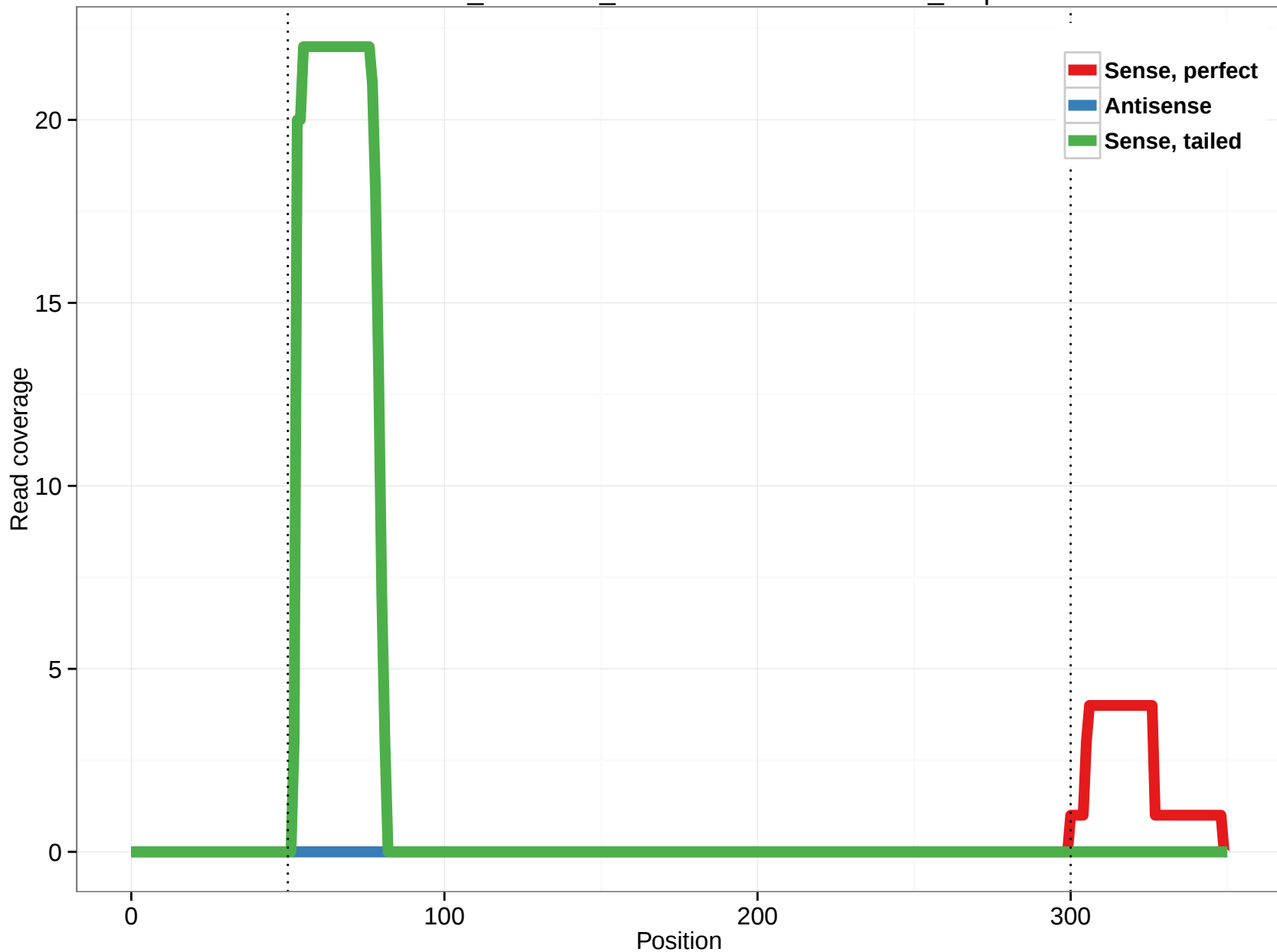
ornAna1_ensGene_ENSOANT00000007976_6.3p
