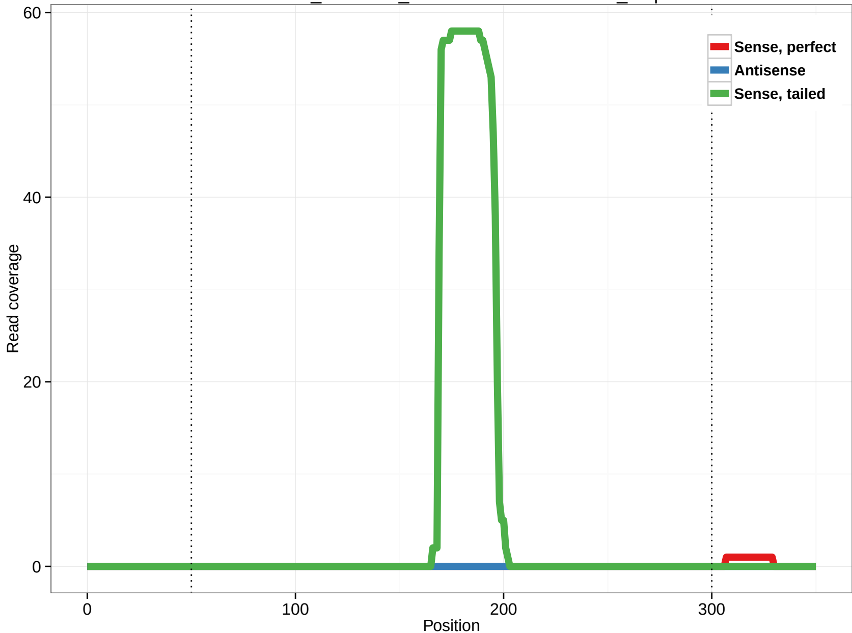
ornAna1_ensGene_ENSOANT00000007886_4.3p
