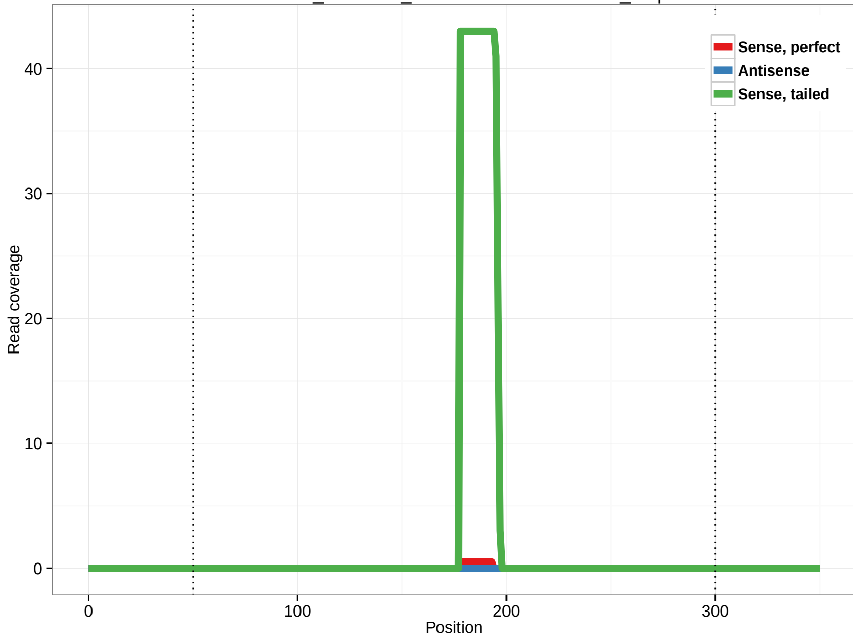
ornAna1_ensGene_ENSOANT00000007886_1.3p
