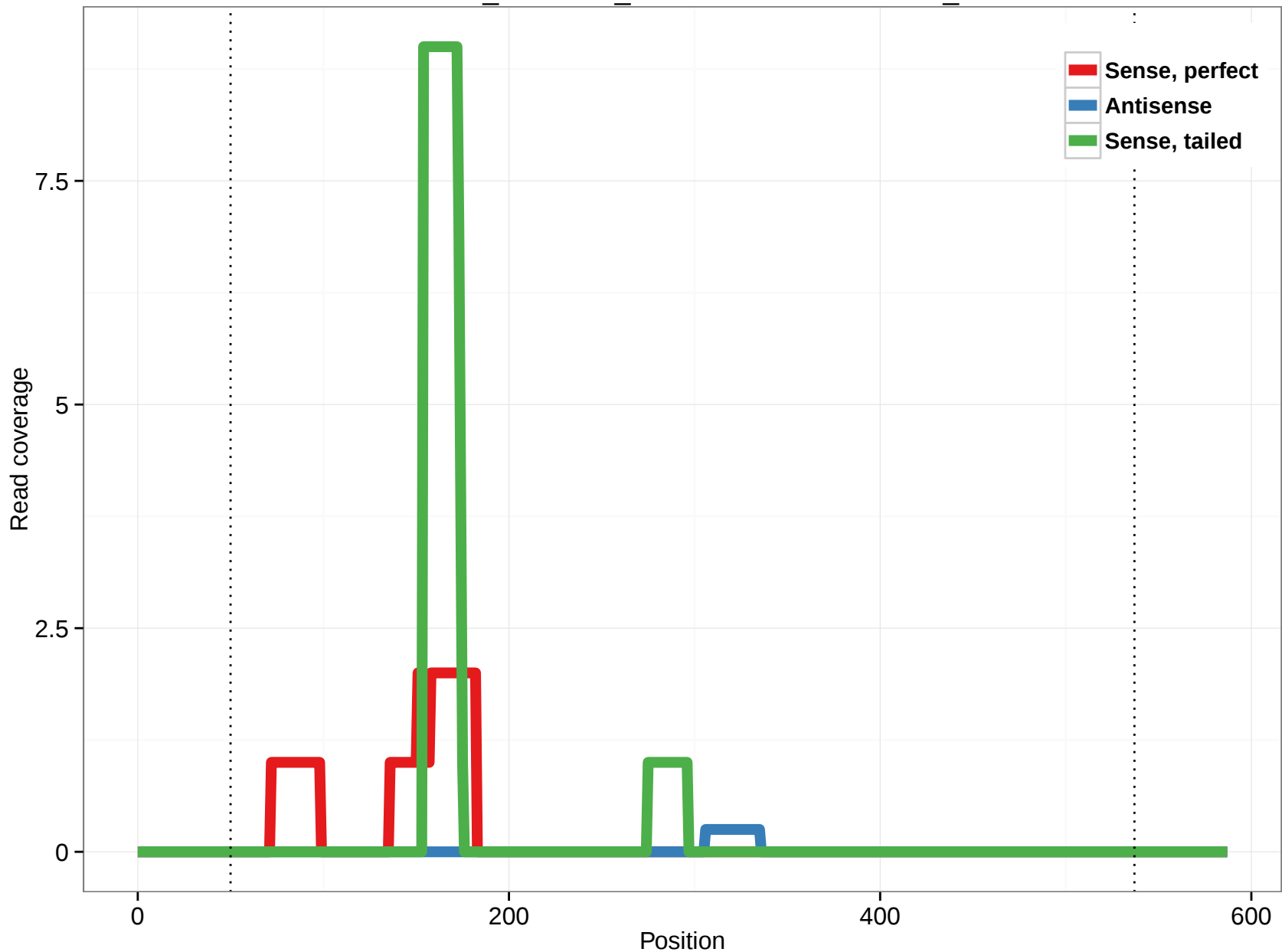
ornAna1_ensGene_ENSOANT00000007872_25
