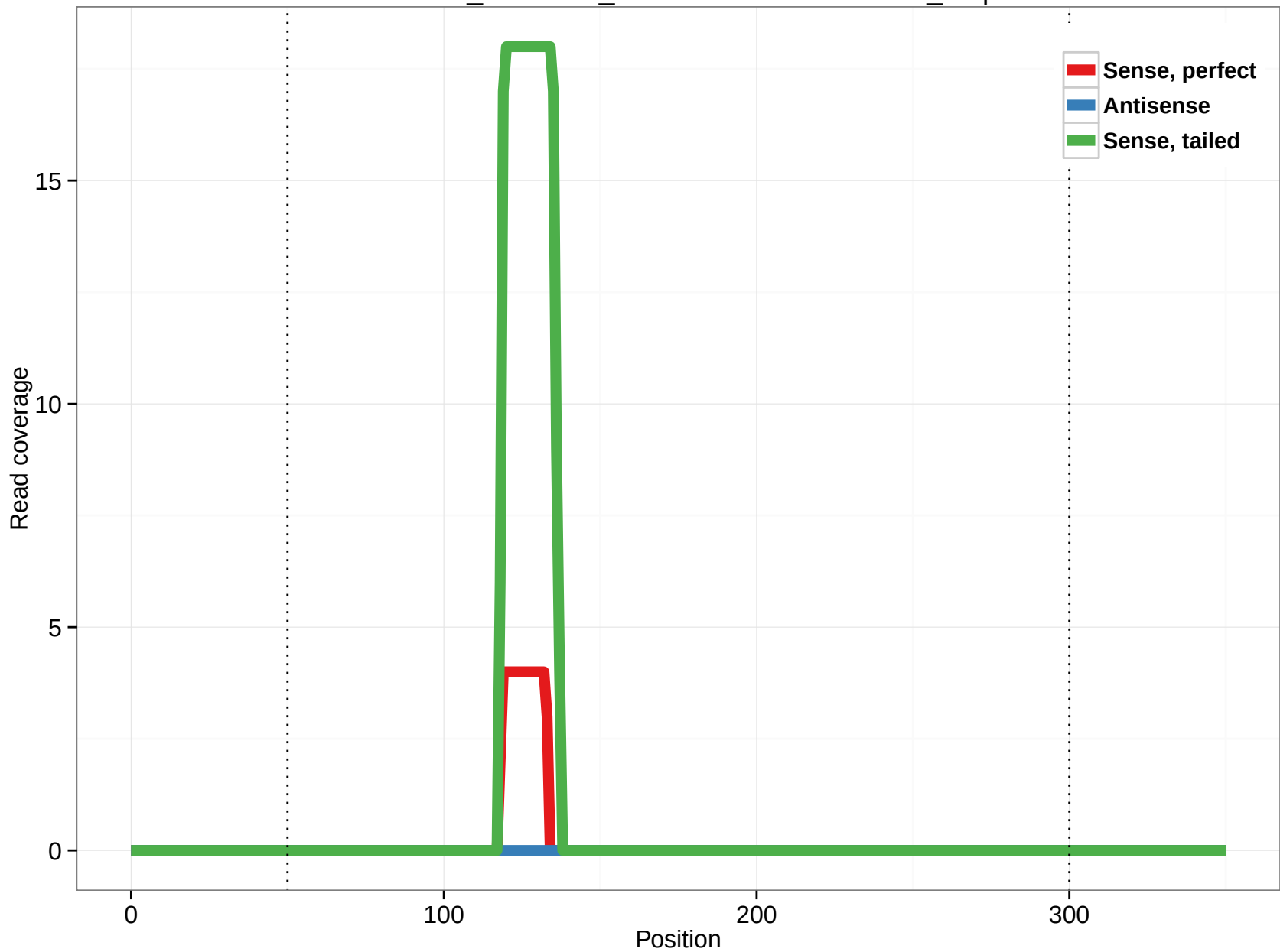
ornAna1_ensGene_ENSOANT00000007864_1.5p
