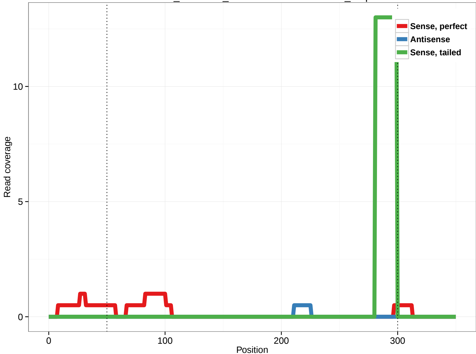
ornAna1_ensGene_ENSOANT00000007852_1.3p
