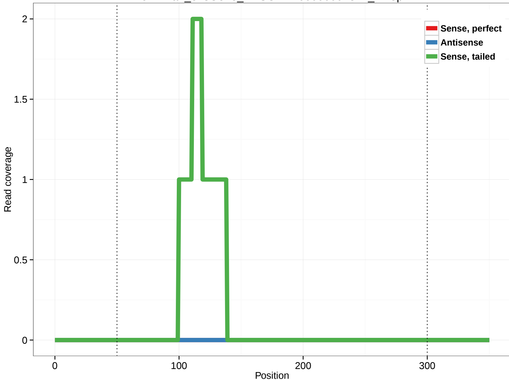
ornAna1_ensGene_ENSOANT00000007811_21.3p
