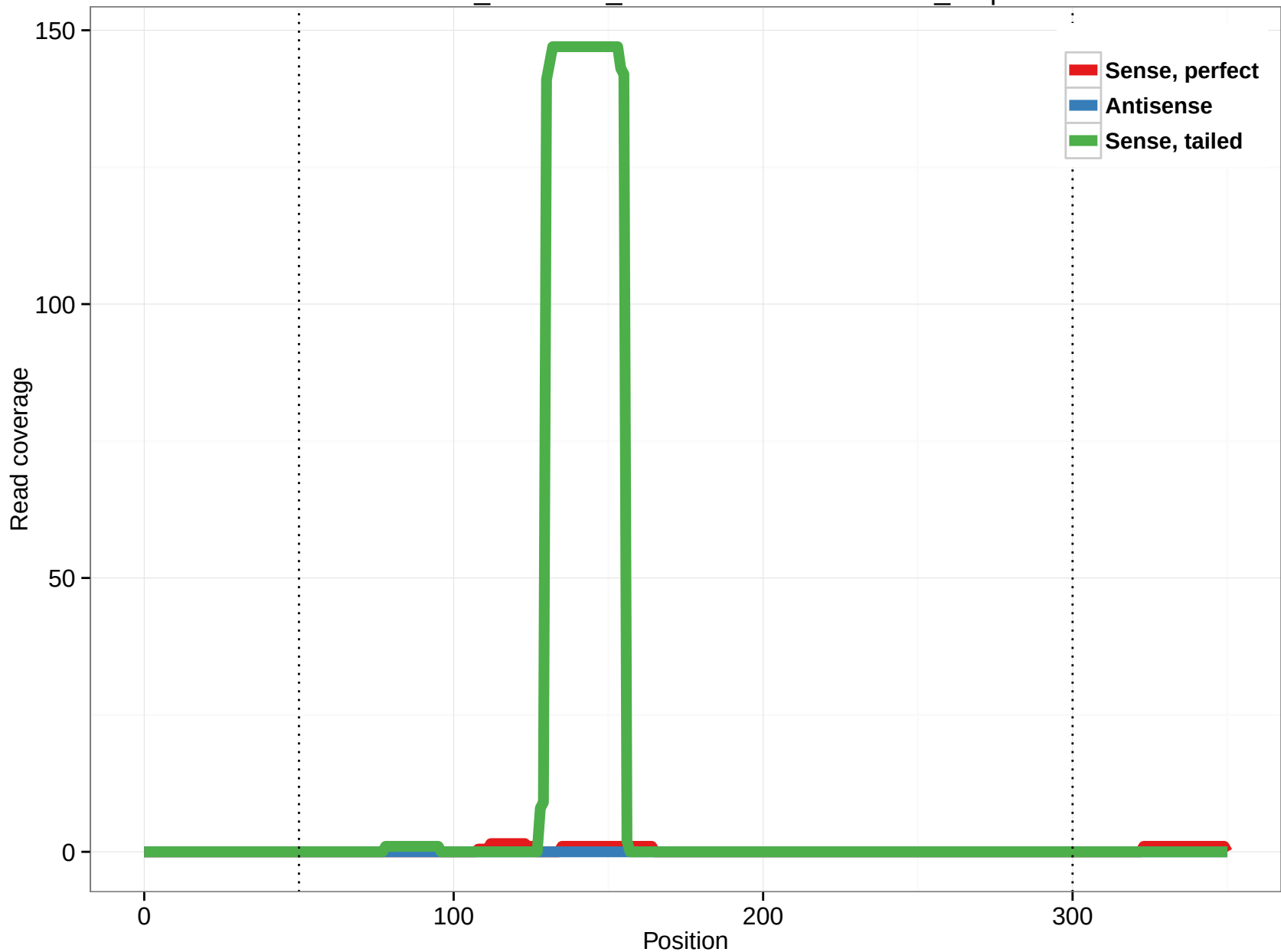
ornAna1_ensGene_ENSOANT00000007783_0.3p
