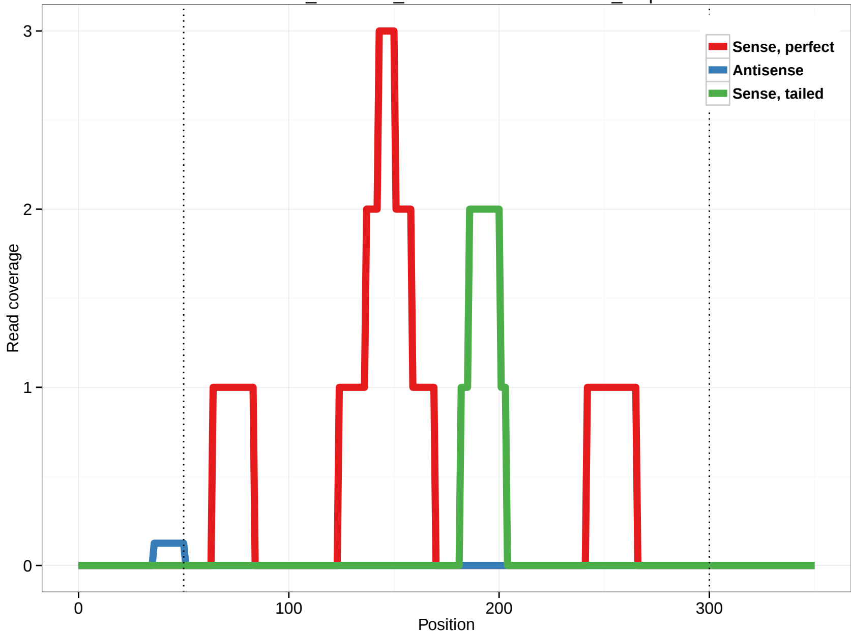
ornAna1_ensGene_ENSOANT00000007648_5.3p
