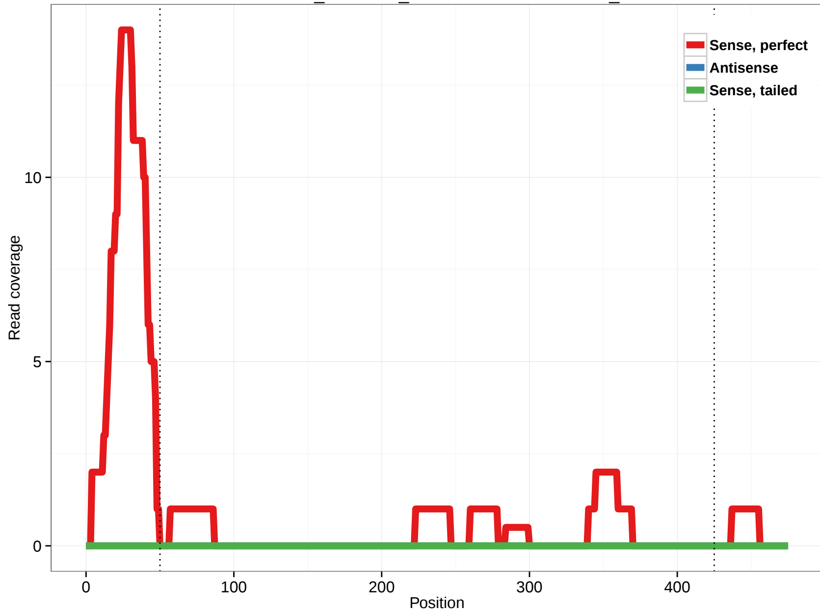
ornAna1_ensGene_ENSOANT00000007648_0
