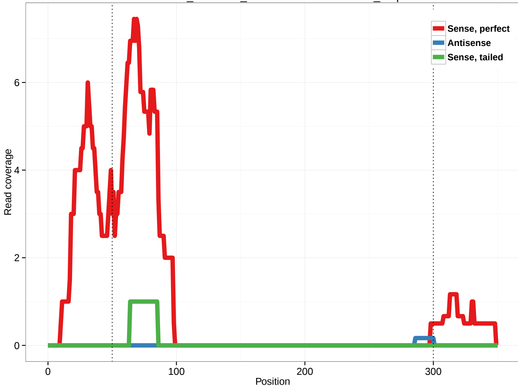
ornAna1_ensGene_ENSOANT00000007613_2.3p
