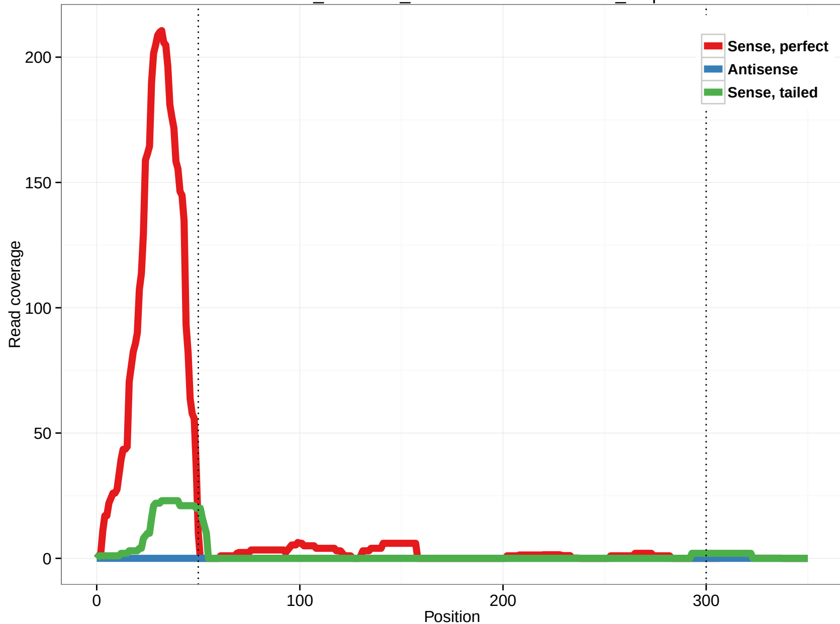
ornAna1_ensGene_ENSOANT00000007581_2.5p
