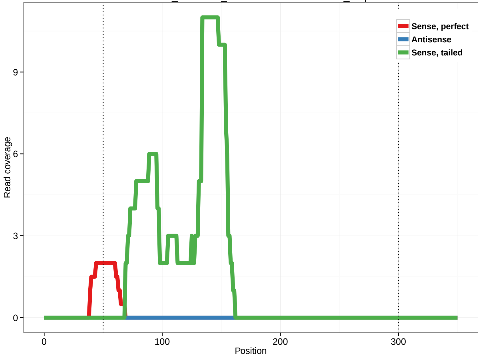
ornAna1_ensGene_ENSOANT00000007560_2.5p
