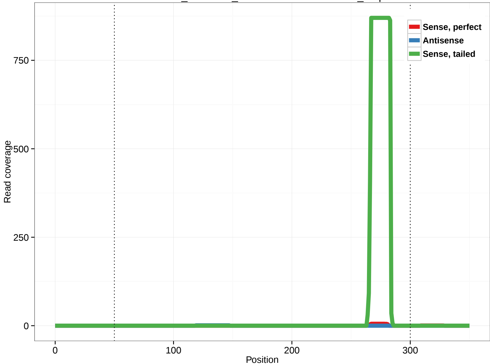
ornAna1_ensGene_ENSOANT00000007555_9.3p
