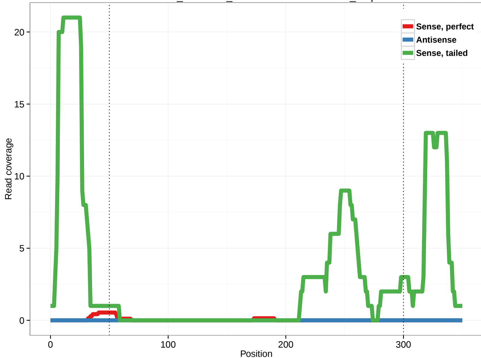
ornAna1_ensGene_ENSOANT00000007540_5.5p
