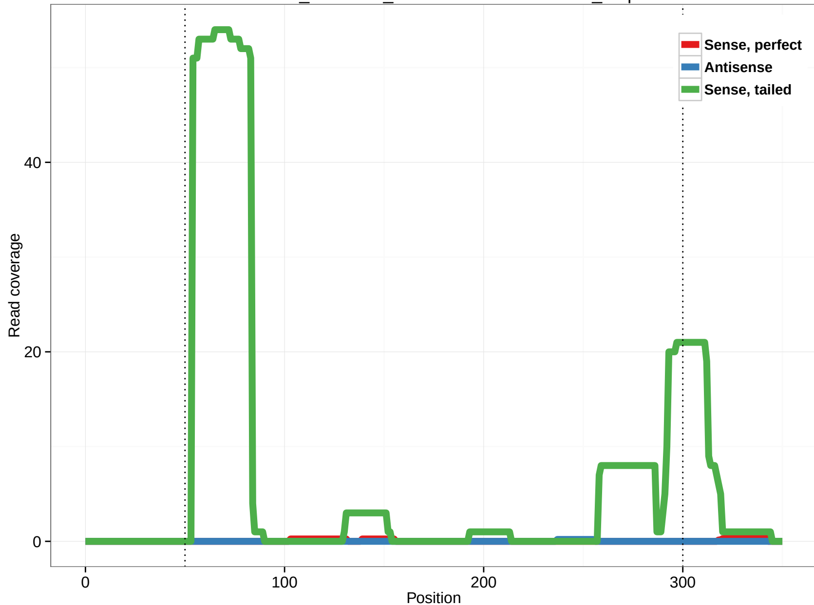
ornAna1_ensGene_ENSOANT00000007540_4.3p
