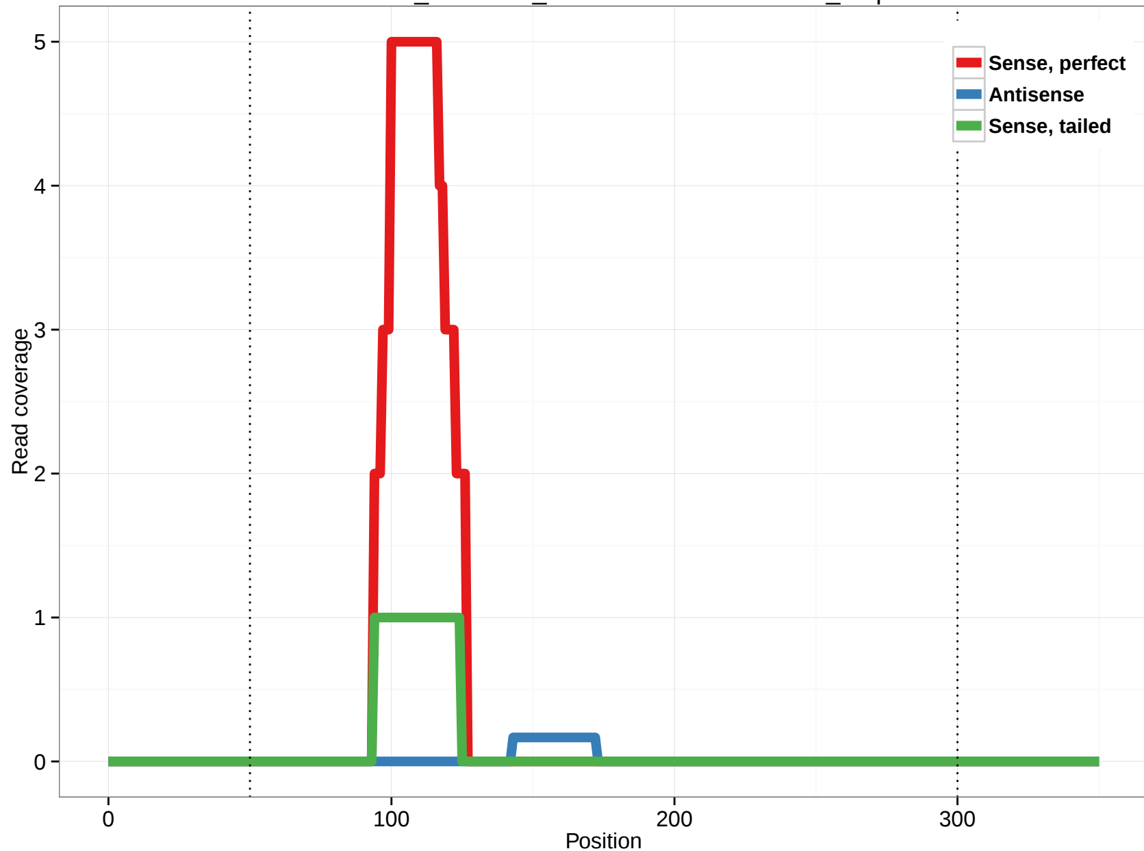
ornAna1_ensGene_ENSOANT00000007531_3.5p
