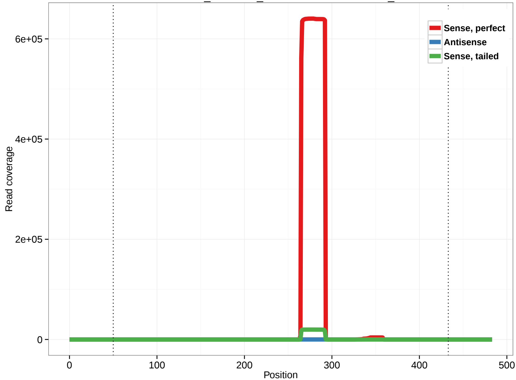
ornAna1_ensGene_ENSOANT00000007401_5
