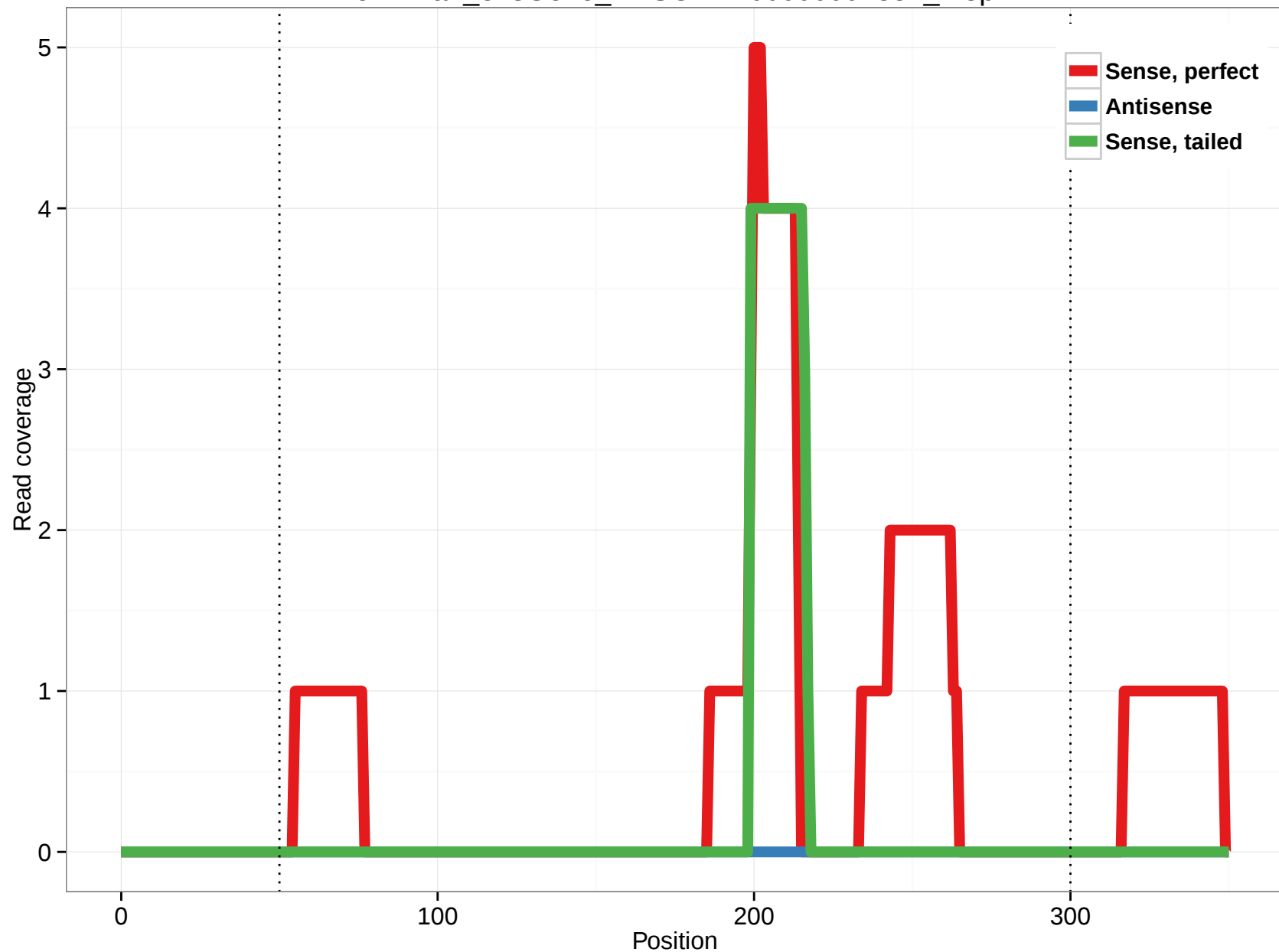
ornAna1_ensGene_ENSOANT00000007384_7.3p
