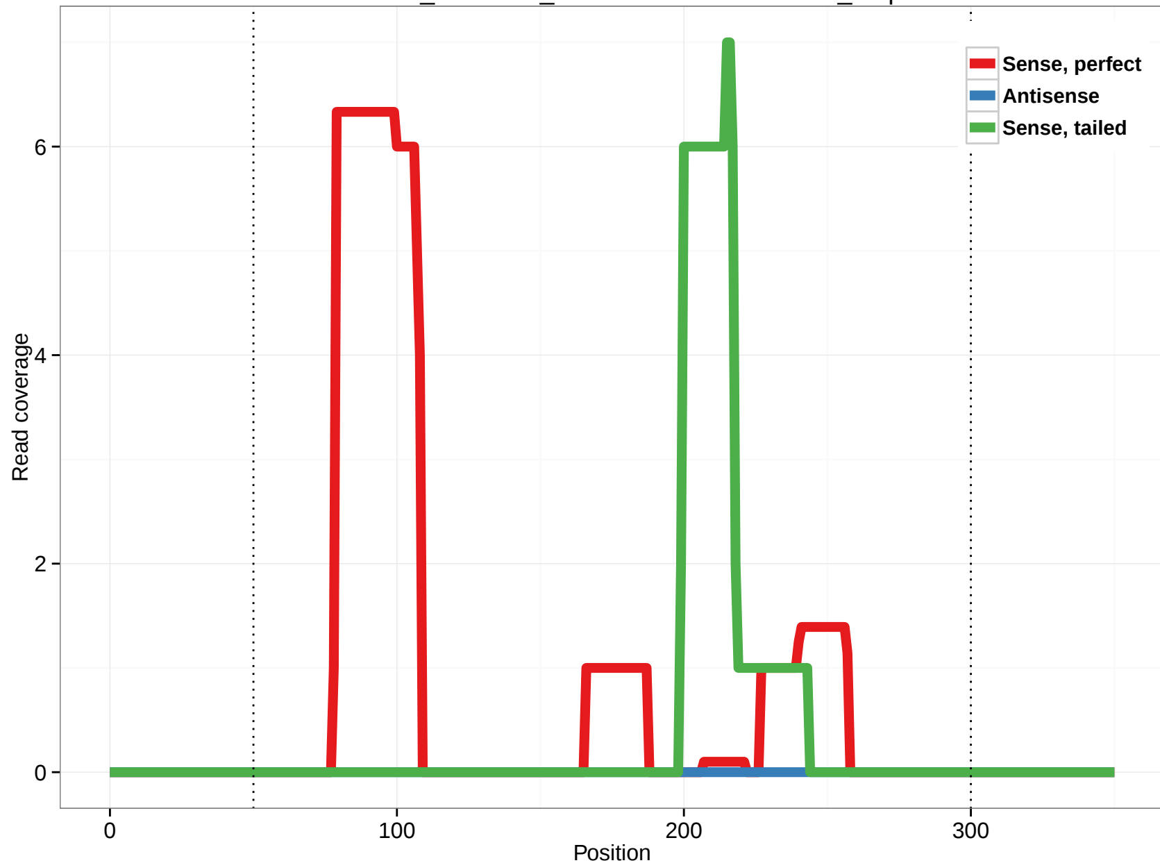
ornAna1_ensGene_ENSOANT00000007384_5.3p
