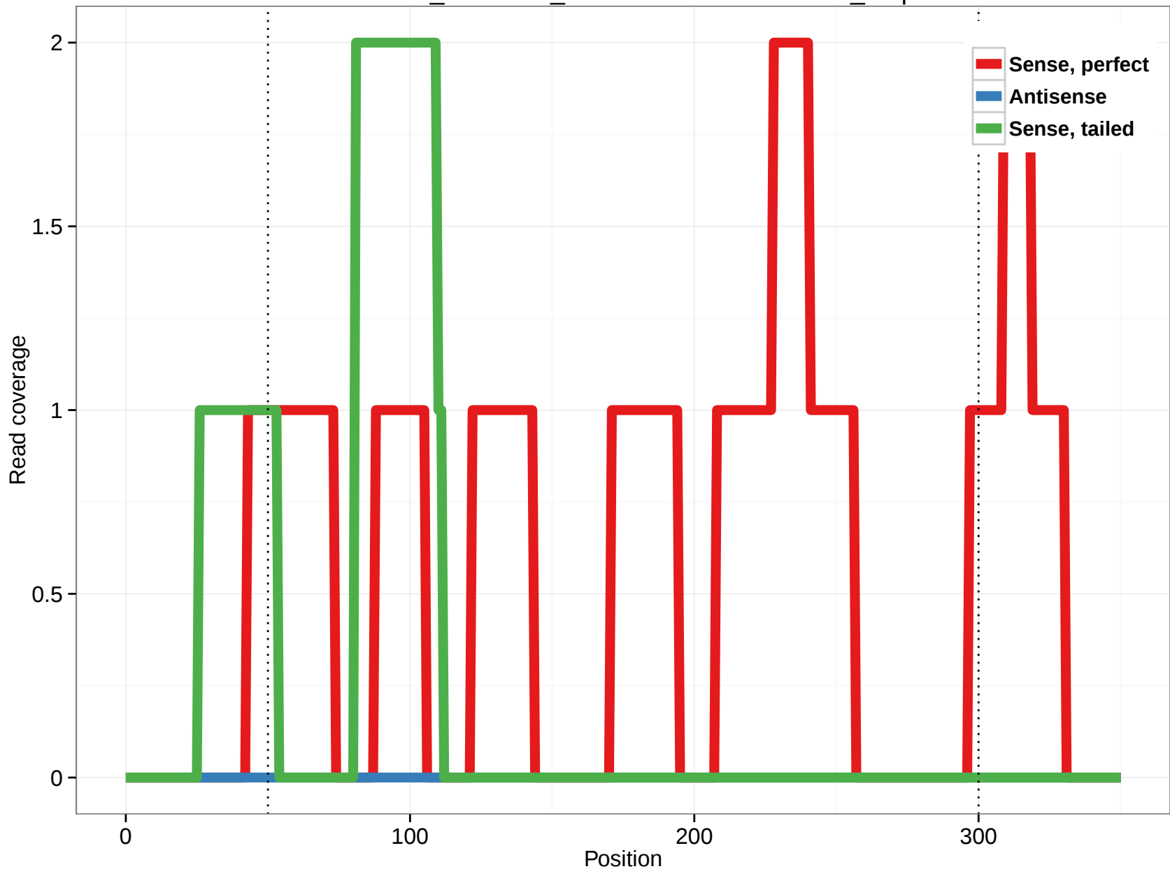
ornAna1_ensGene_ENSOANT00000007381_2.5p
