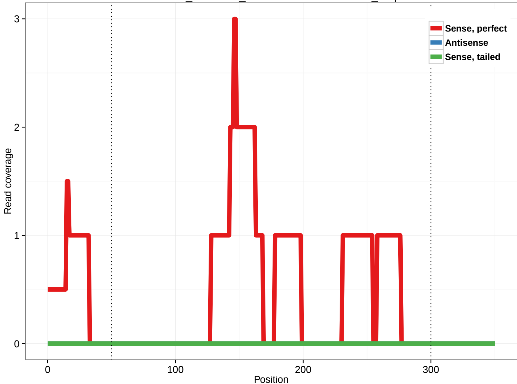
ornAna1_ensGene_ENSOANT00000007346_1.5p
