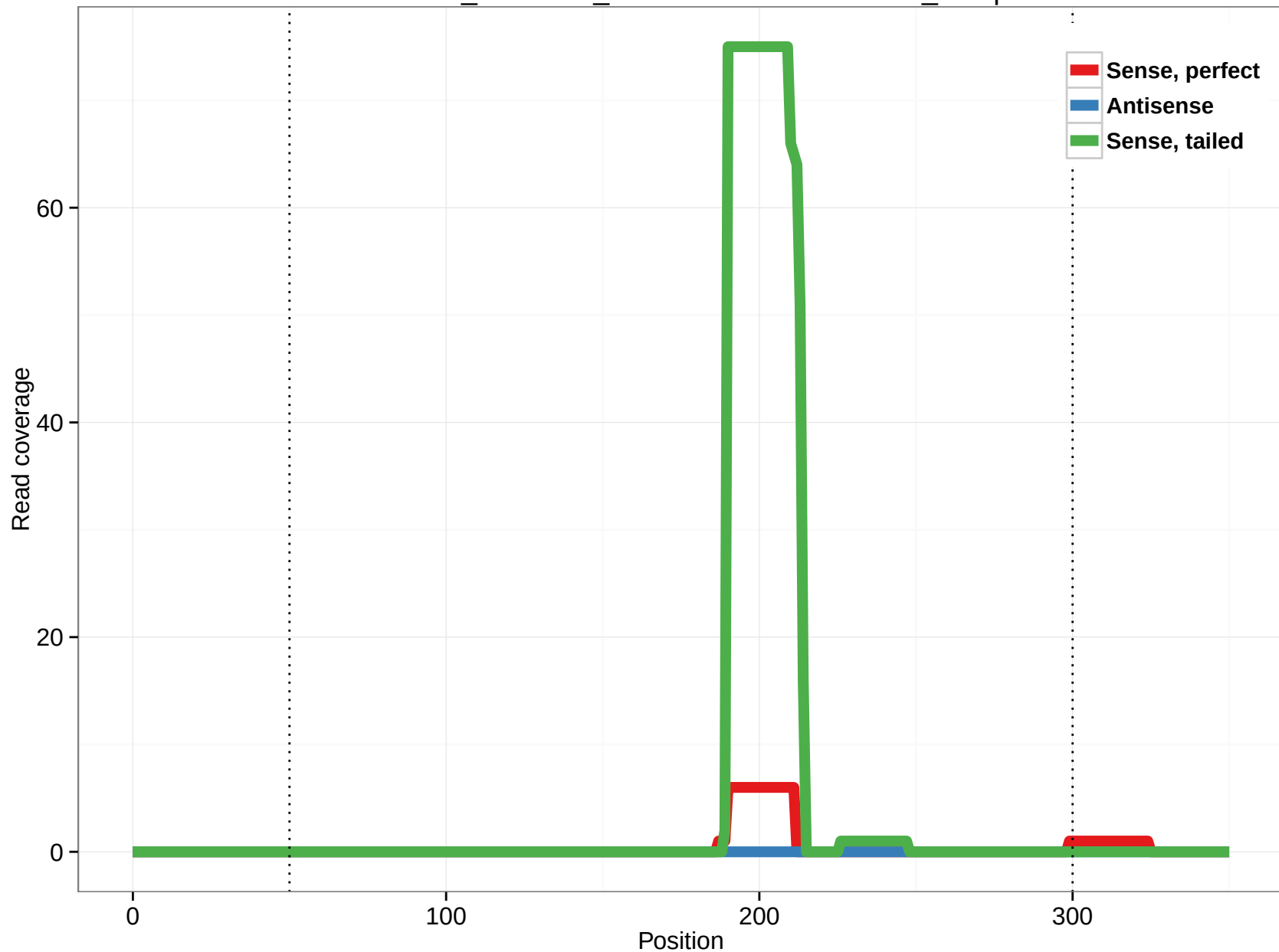
ornAna1_ensGene_ENSOANT00000007341_14.3p
