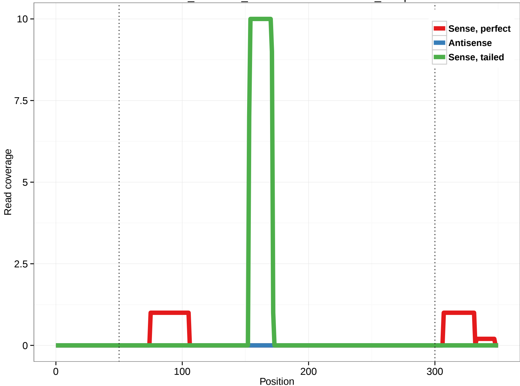
ornAna1_ensGene_ENSOANT00000007320_12.3p
