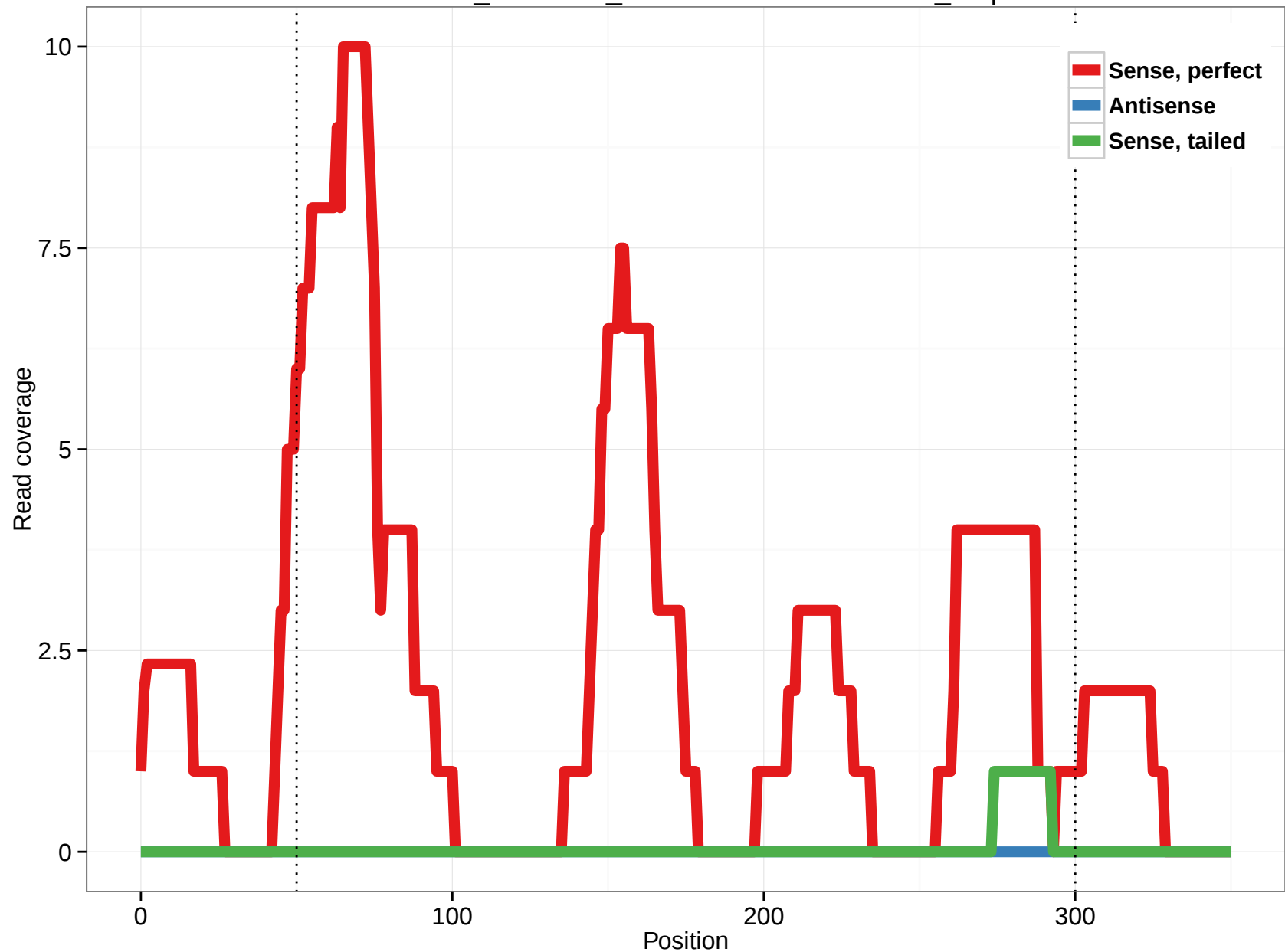
ornAna1_ensGene_ENSOANT00000007314_6.5p
