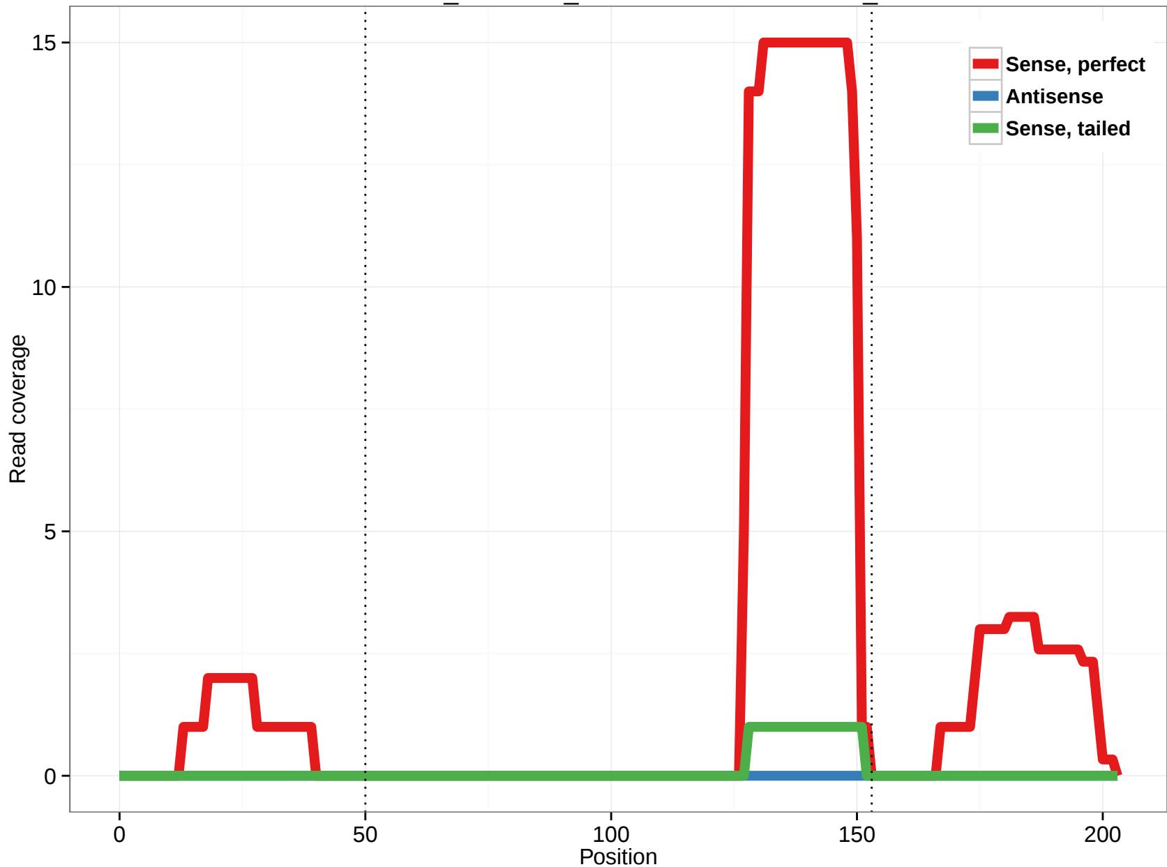
ornAna1_ensGene_ENSOANT00000007251_0
