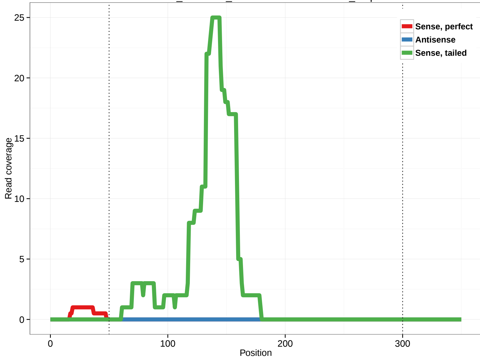
ornAna1_ensGene_ENSOANT00000007223_1.5p
