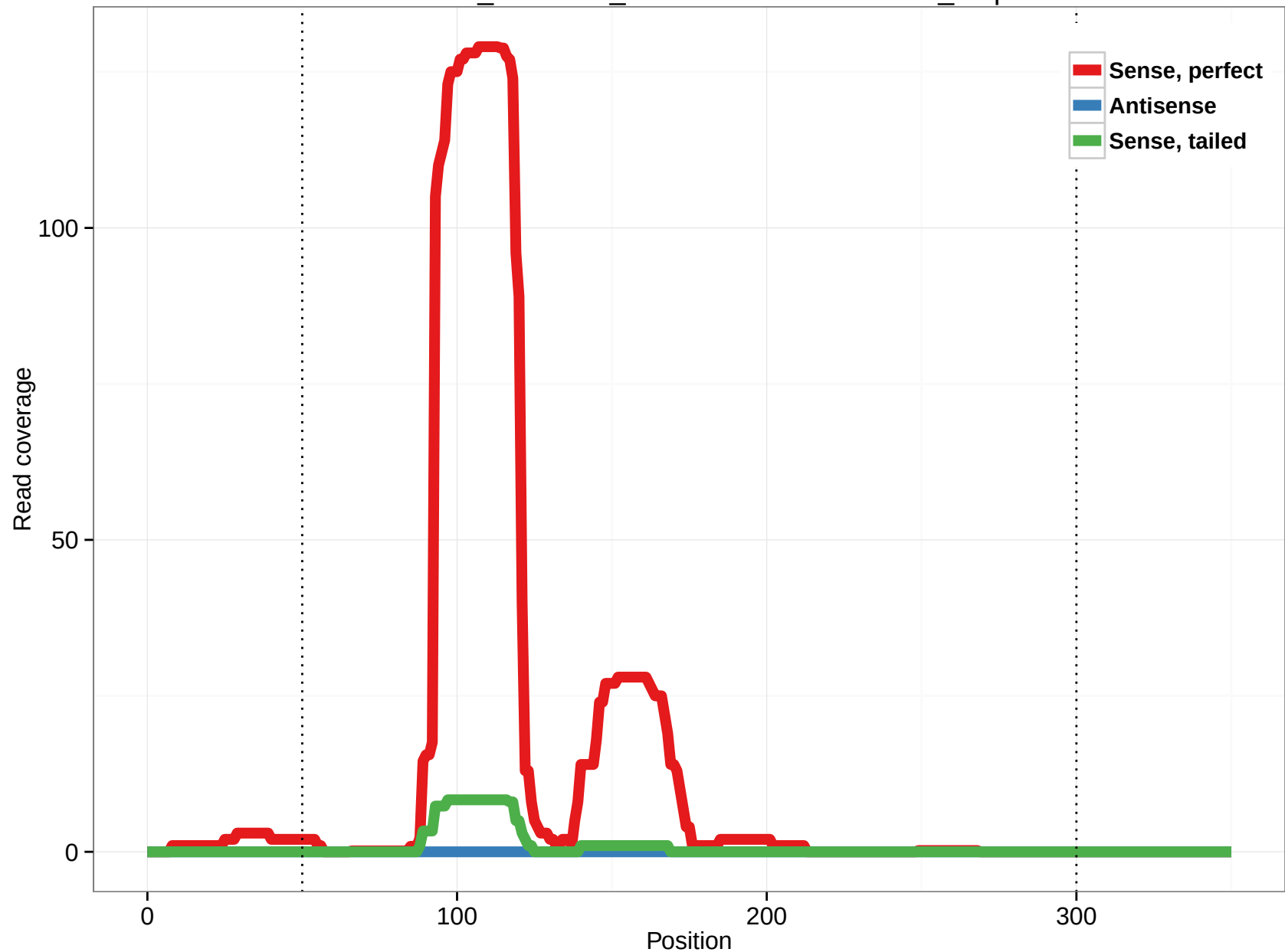
ornAna1_ensGene_ENSOANT00000007184_0.3p
