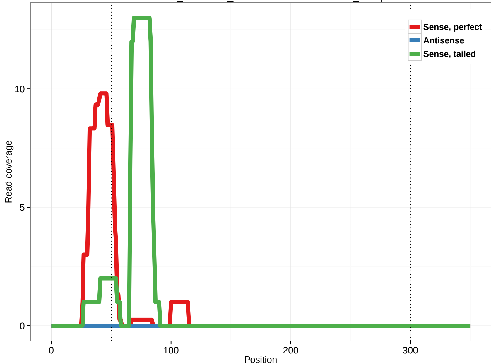
ornAna1_ensGene_ENSOANT00000007105_41.3p
