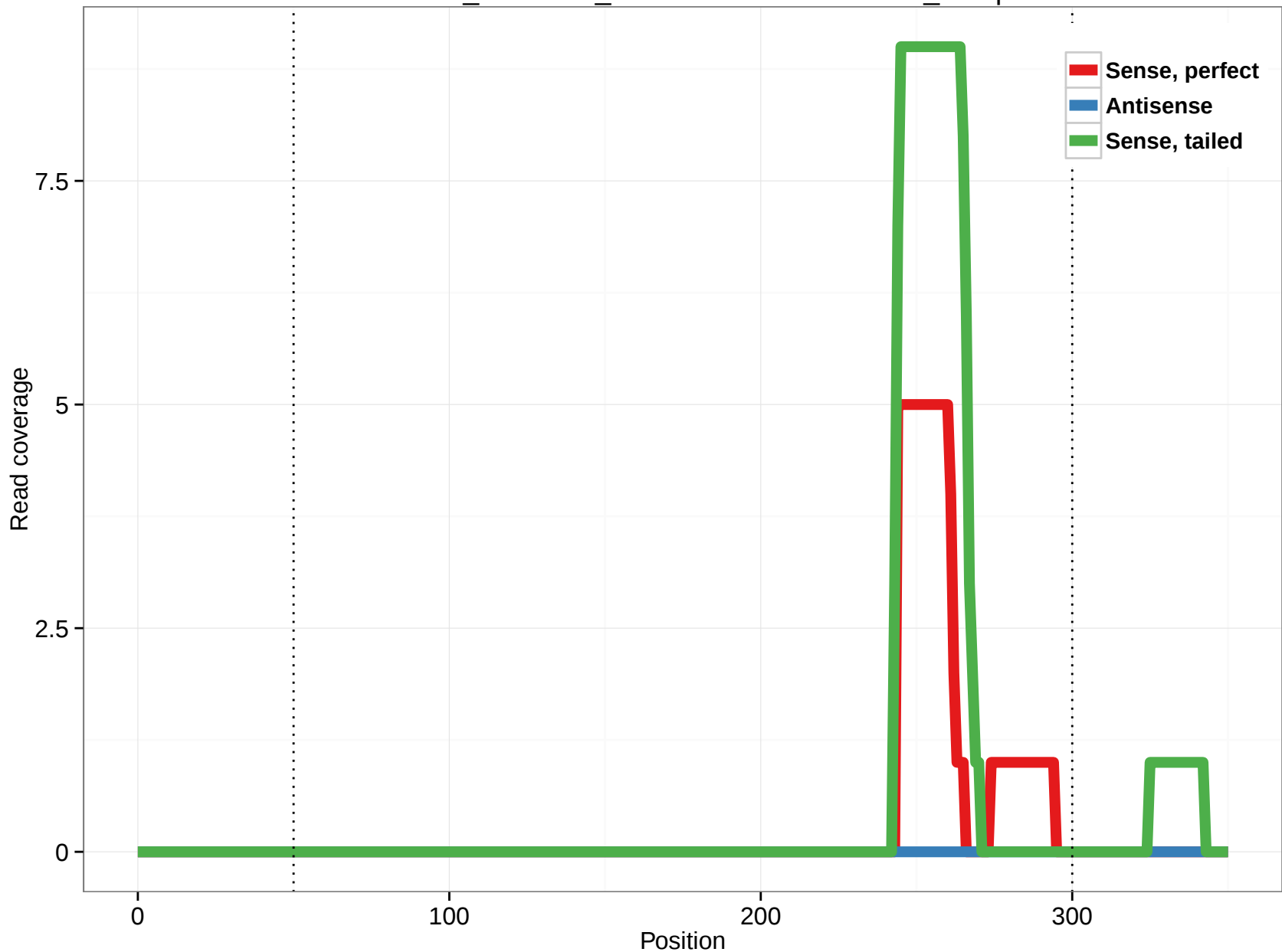
ornAna1_ensGene_ENSOANT00000007090_13.3p
