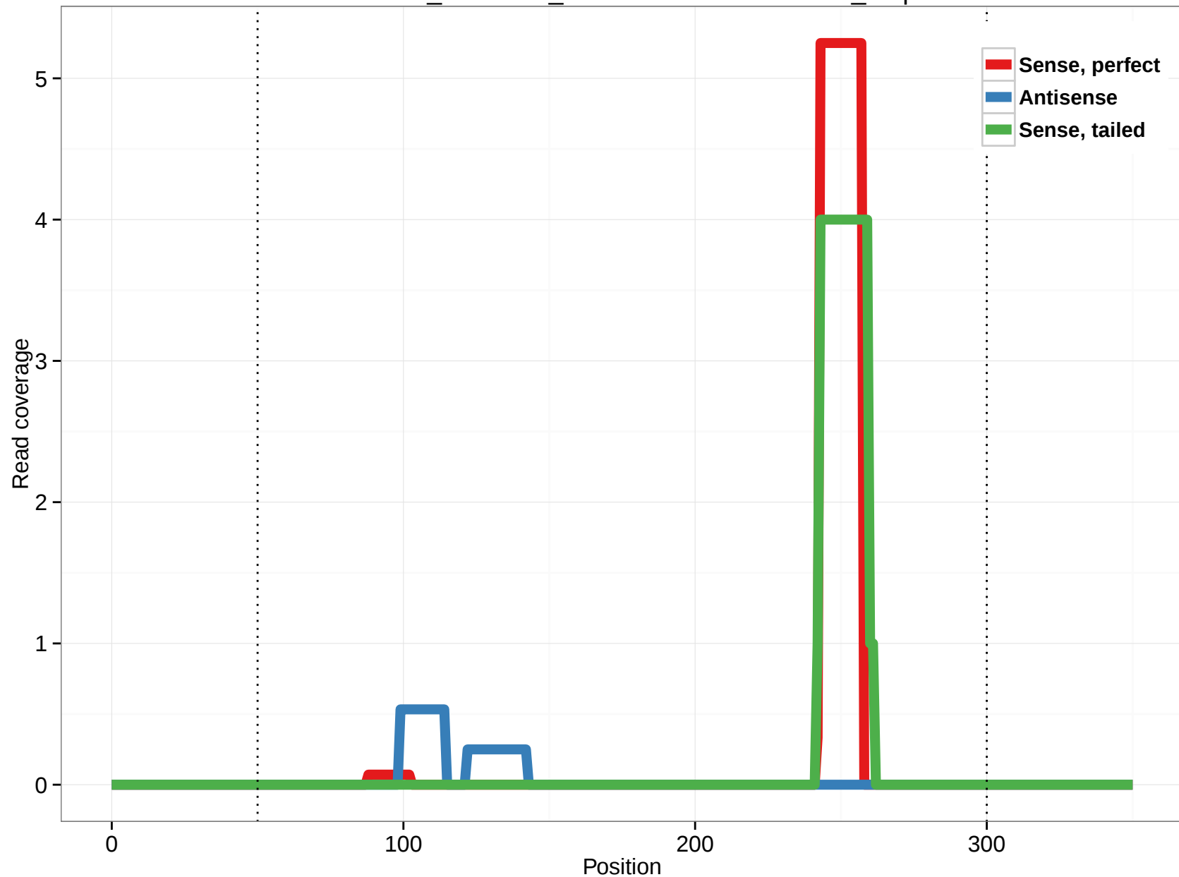
ornAna1_ensGene_ENSOANT00000006980_0.3p
