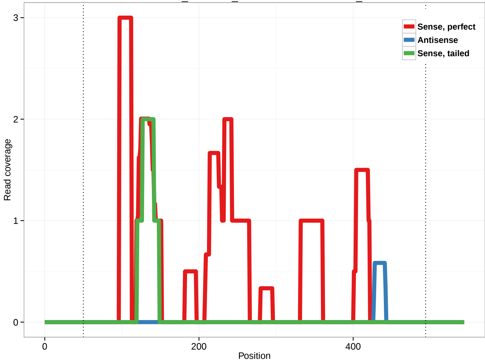
ornAna1_ensGene_ENSOANT00000006957_6
