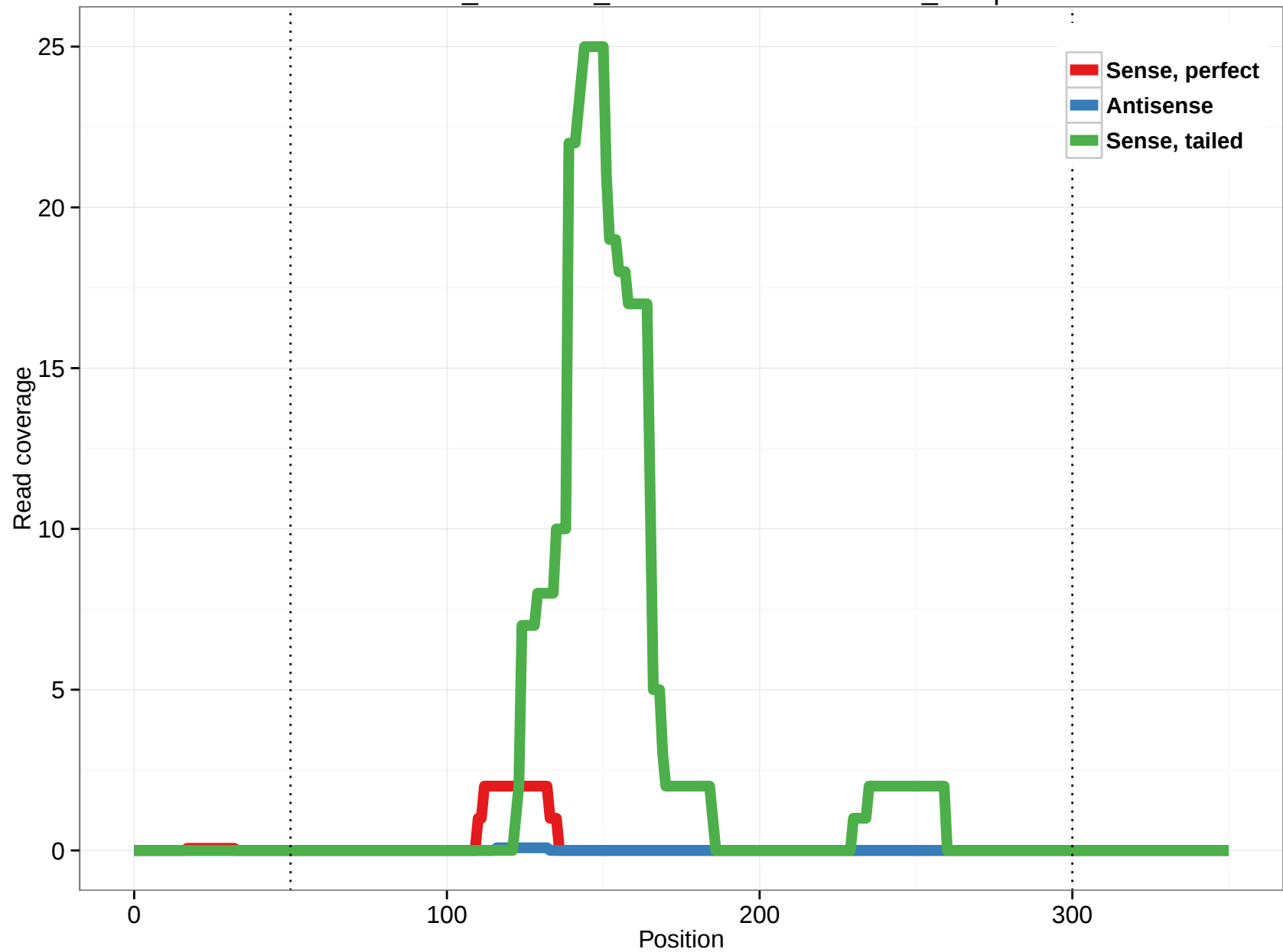
ornAna1_ensGene_ENSOANT00000006947_15.5p
