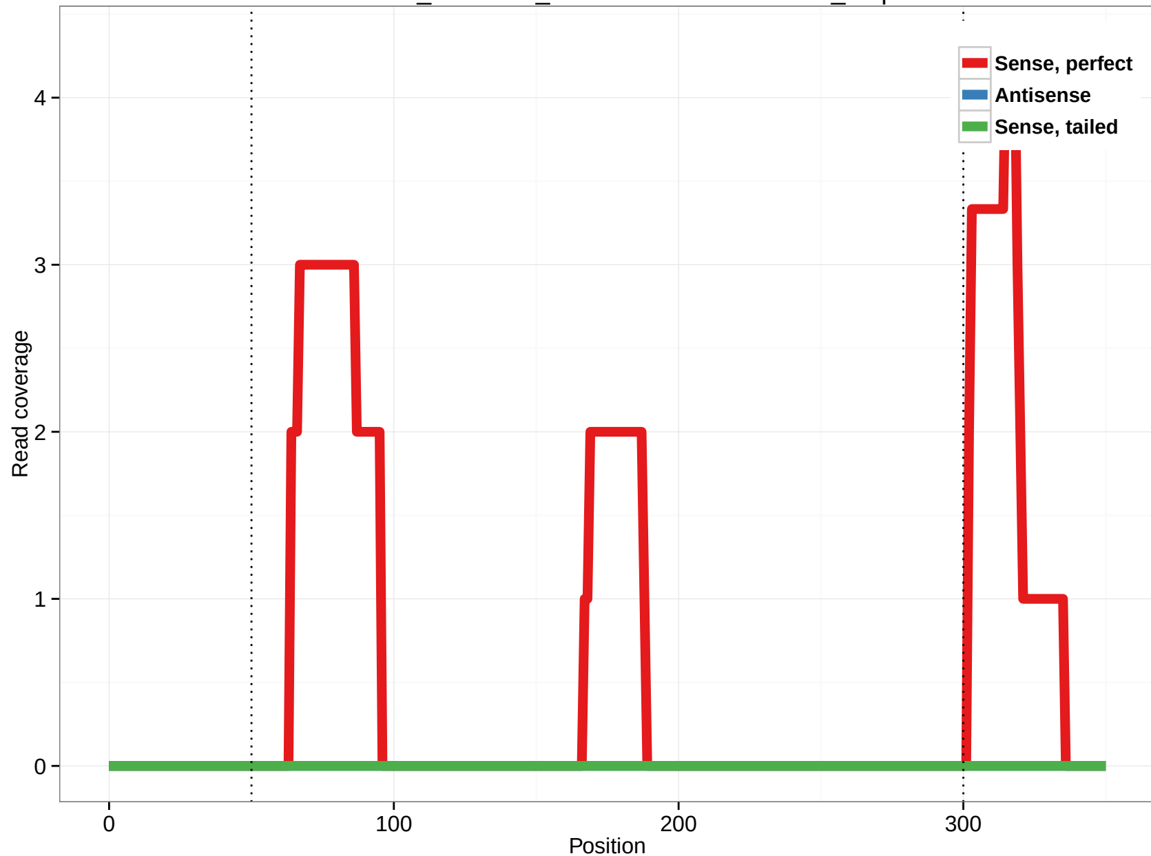
ornAna1_ensGene_ENSOANT00000006945_0.3p
