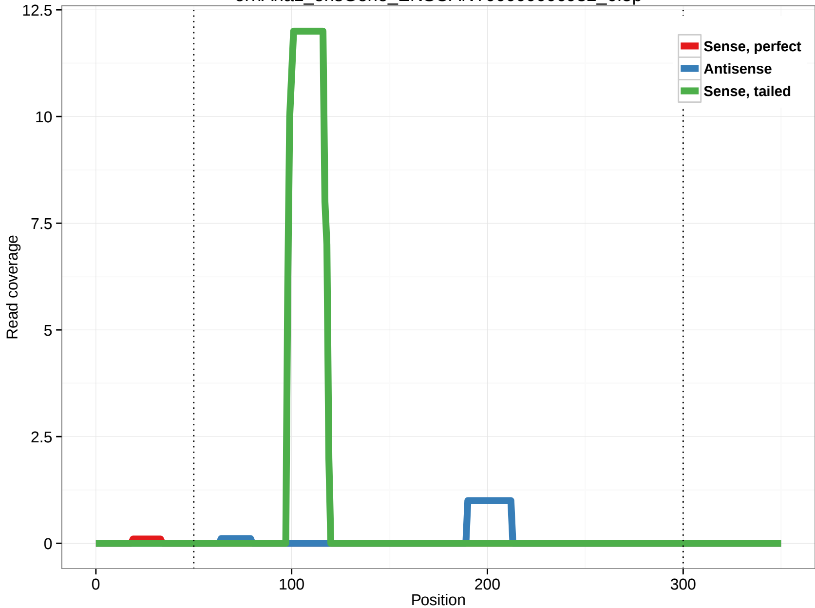
ornAna1_ensGene_ENSOANT00000006932_6.5p
