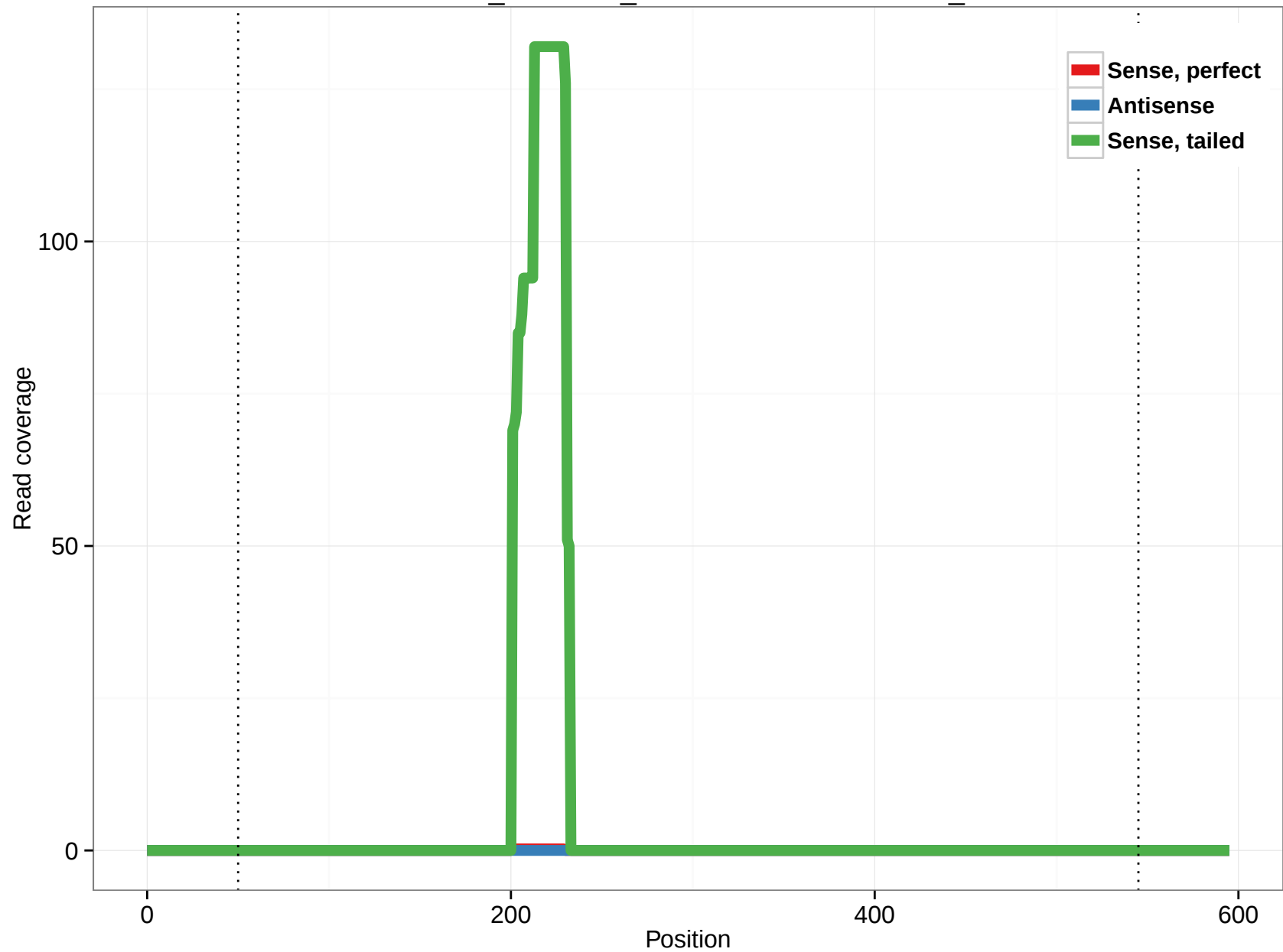
ornAna1_ensGene_ENSOANT00000006870_12
