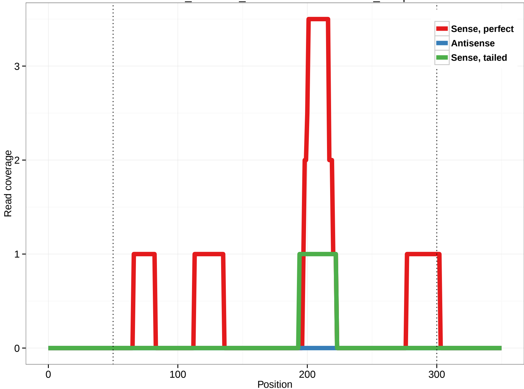
ornAna1_ensGene_ENSOANT00000006856_23.5p
