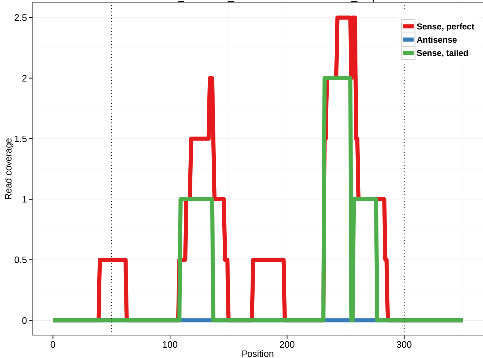
ornAna1_ensGene_ENSOANT00000006807_0.5p
