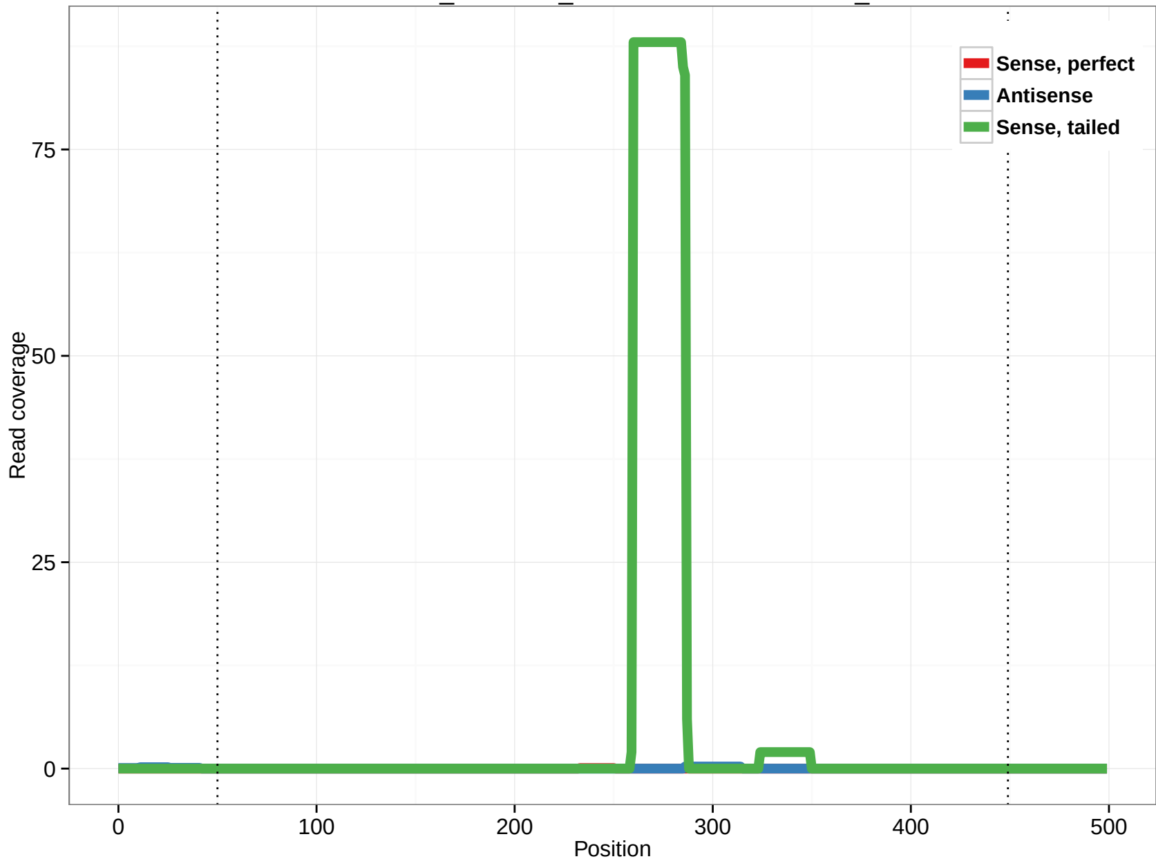
ornAna1_ensGene_ENSOANT00000006774_0
