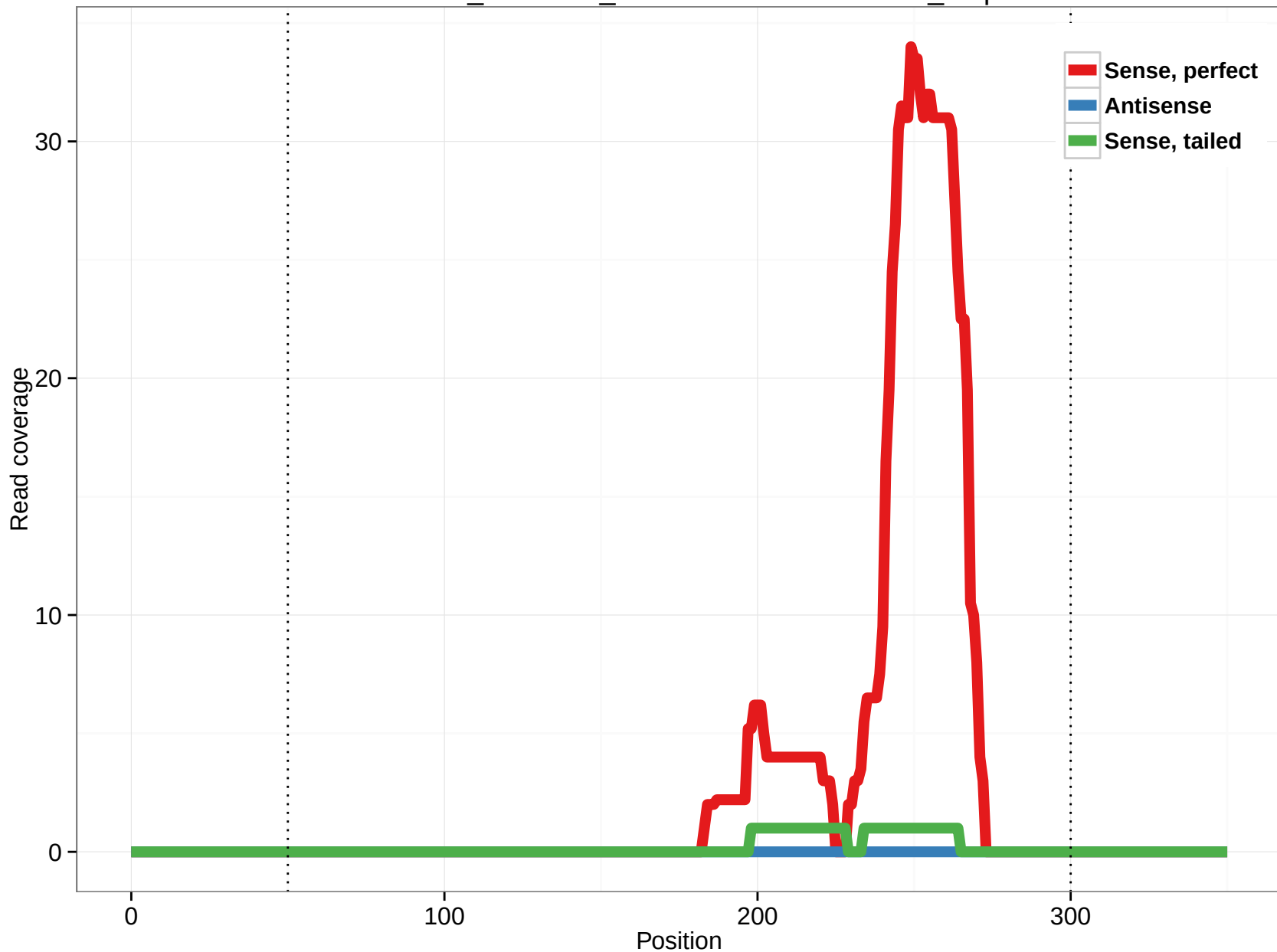
ornAna1_ensGene_ENSOANT00000006724_0.5p
