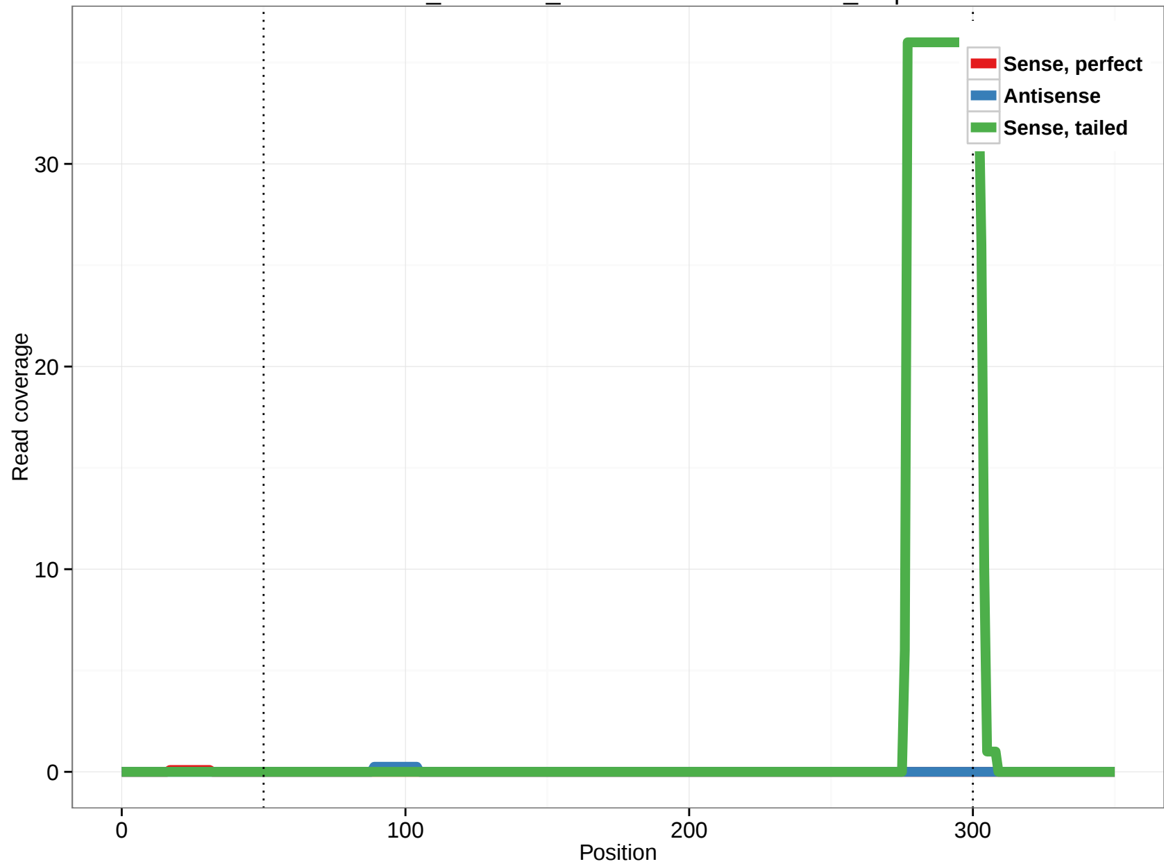
ornAna1_ensGene_ENSOANT00000006659_2.5p
